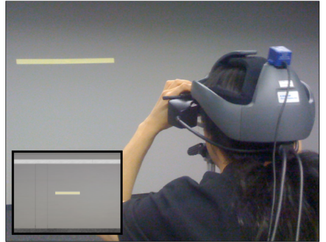
Figure 2: Picture taken during the psychophysical calibration process. A participant at a fixed position compares the size of the horizontal stripe in the real world with the virtual stripe displayed on the HMD (see inset).
