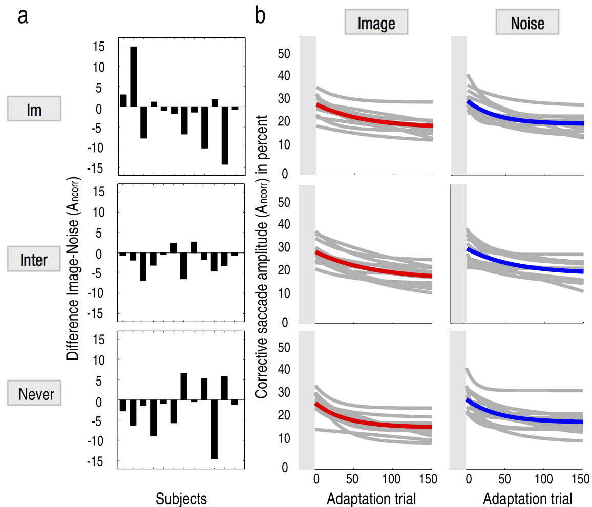
Figure 5. (a) Difference (image–noise) in mean corrective saccades amplitudes in late adaptation ( A_{\text{corr}} ) in the three masking conditions for all individual subjects. (b) Exponential fits of single subjects (gray) and averaged corrective saccades' amplitudes towards images (red) and noise (blue).
