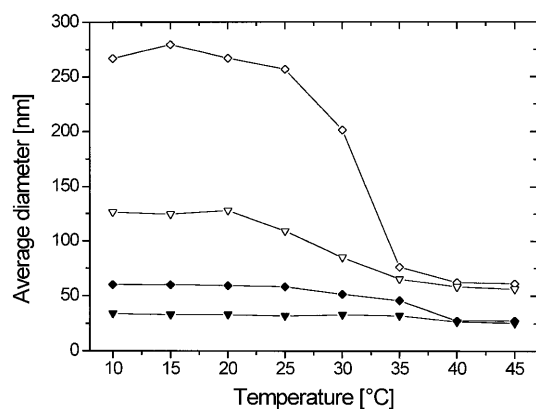
Fig. 6 Dependence of the average hydrodynamic diameter of the nanogels on temperature (open diamonds: 5-1-30; open down triangles: 10-1-30; filled diamonds: 5-2-30; filled down triangles: 10-2-30)
