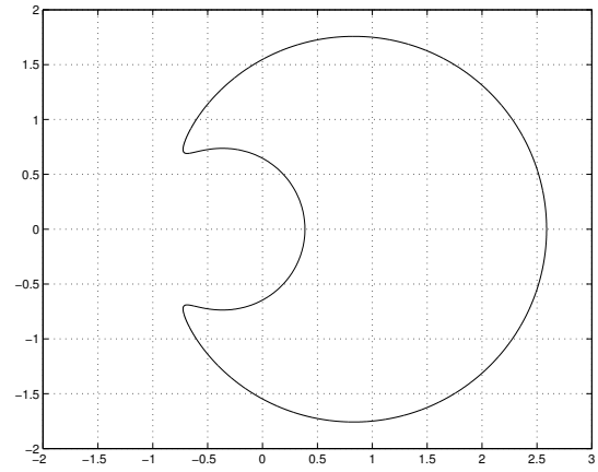
(b) Boundary of the inclusion set after the second Möbius transformation
