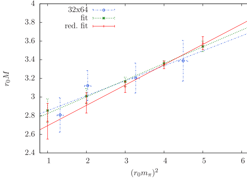
Figure 6.2.: The gluino-gluon mass extrapolated to the infinite volume limit as a function of the squared mass of the adjoint pion in units of the Sommer scale and the mass at the largest lattice volume at different values of \kappa
