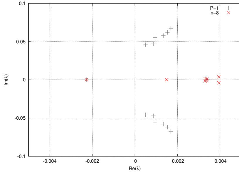
Figure 5.7.: Lowest 10 eigenvalues of D on the lattice of volume 32^3 \times 64 with \beta = 1.75 and \kappa = 0.1495 calculated using the polynomial in the figure. Grey points are 20 eigenvalues calculated by ARPACK in LR mode.
