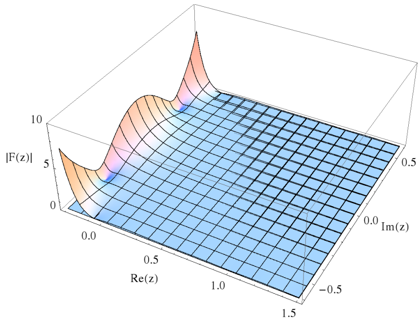
Figure 5.25.: Magnitude of the 20th Faber polynomial corresponding to the SC mapping illustrated in figure 5.22
