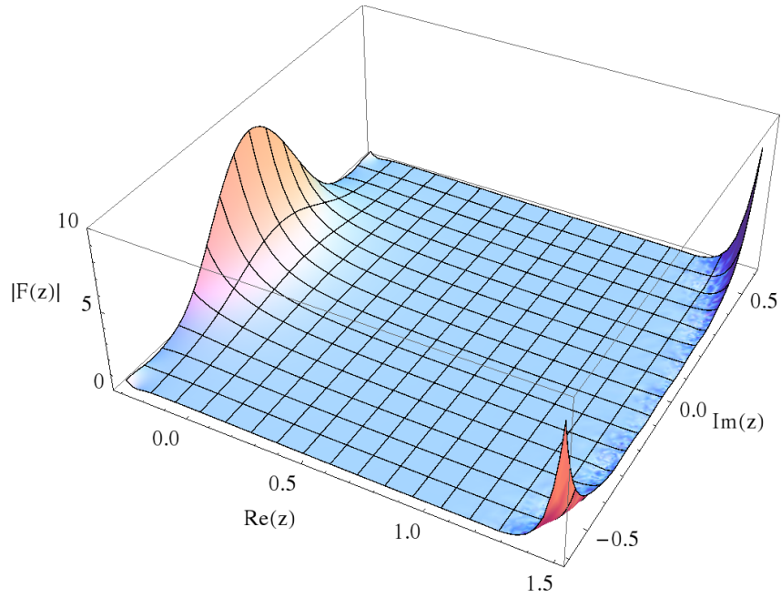
Figure 5.17.: Magnitude of the 30th Faber polynomial corresponding to the BW mapping illustrated in figure 5.14
