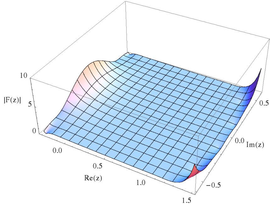
Figure 5.16.: Magnitude of the 20th Faber polynomial corresponding to the BW mapping illustrated in figure 5.14
