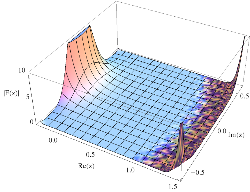
Figure 5.18.: Magnitude of the 40th Faber polynomial corresponding to the BW mapping illustrated in figure 5.14
