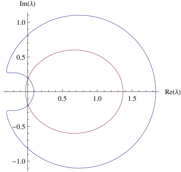
Figure 5.12.: Boundary of the BW mapping with \epsilon = 0.3 and \phi = \pi/2 , scaled in accordance with the eigenspectrum represented by the purple ellipse
