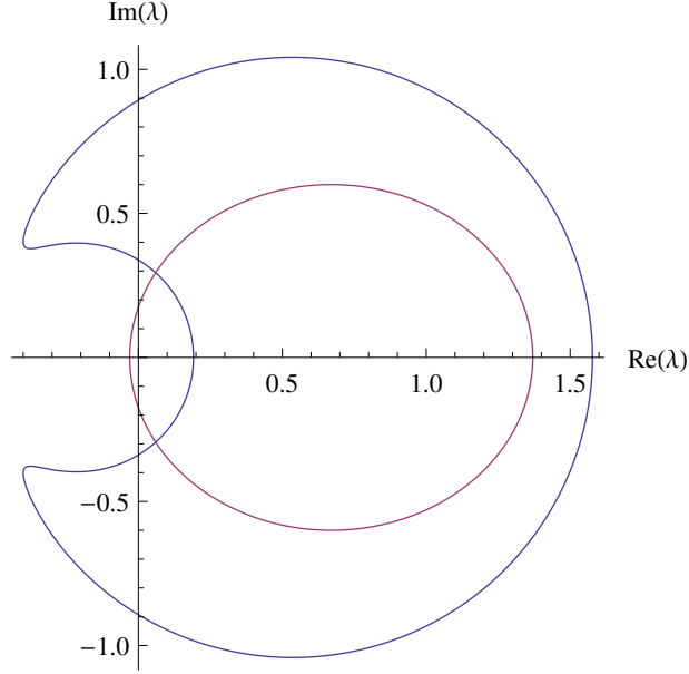
Figure 5.14.: Boundary of the BW mapping with \epsilon = 0.22 and \phi = \pi/2 , scaled in accordance with the eigenspectrum represented by the purple ellipse
