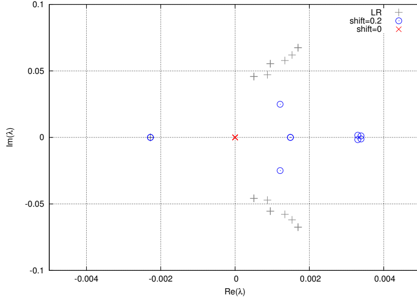
Figure 5.21.: Lowest 10 eigenvalues of D on the lattice of volume 32^3 \times 64 with \beta = 1.75 and \kappa = 0.1495 calculated using F_{40}^{0.22}(z) and F_{40}^{0.22}(z - 0.2) . Grey points are 20 eigenvalues calculated by ARPACK in LR mode. The red cross means that no eigenvalues could be calculated using F_{40} due to numerical instabilities seen in Fig. 5.18.
