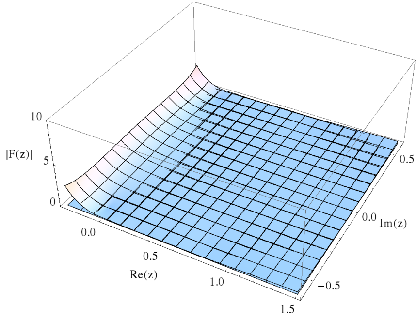
Figure 5.24.: Magnitude of the 10th Faber polynomial corresponding to the SC mapping illustrated in figure 5.22
