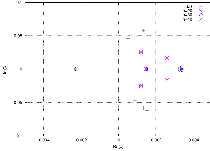
Figure 5.28.: Lowest 10 eigenvalues of D on the lattice of volume 32^3 \times 64 with \beta = 1.75 and \kappa = 0.1495 calculated using F_{20}^{SC}(z) and F_{30}^{SC}(z) . Grey points are 20 eigenvalues calculated by ARPACK in LR mode. The red cross means that no eigenvalues could be calculated using F_{40} due to numerical instabilities seen in figure 5.27.
