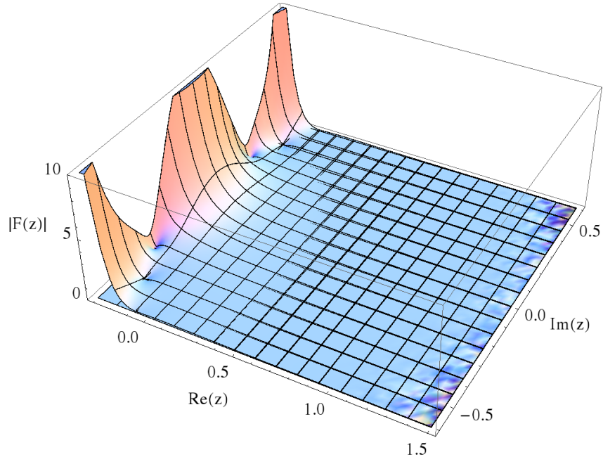
Figure 5.26.: Magnitude of the 30th Faber polynomial corresponding to the SC mapping illustrated in figure 5.22
