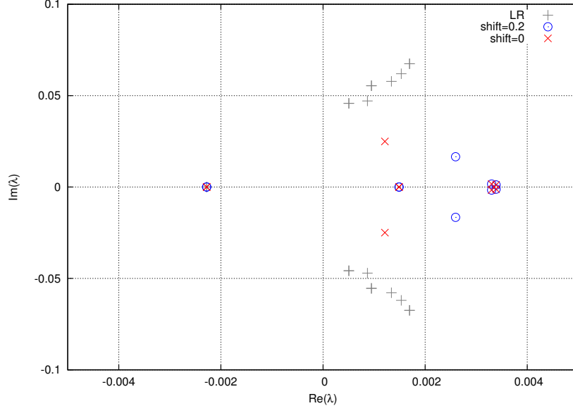
Figure 5.20.: Lowest 10 eigenvalues of D on the lattice of volume 32^3 \times 64 with \beta = 1.75 and \kappa = 0.1495 calculated using F_{40}^{0.3}(z) and F_{40}^{0.3}(z - 0.2) . Grey points are 20 eigenvalues calculated by ARPACK in LR mode
