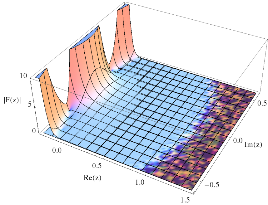
Figure 5.27.: Magnitude of the 40th Faber polynomial corresponding to the SC mapping illustrated in figure 5.22
