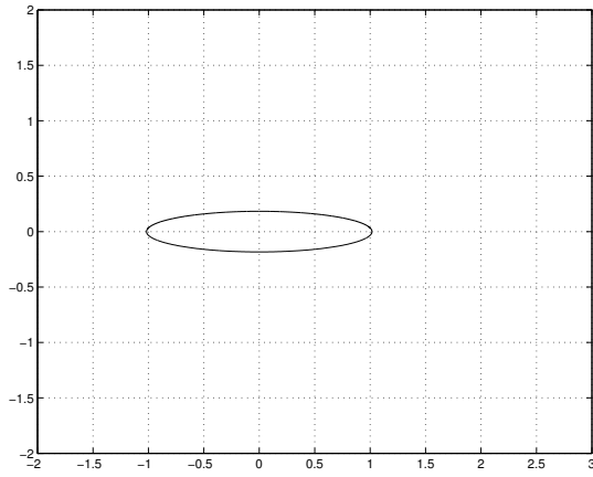
(a) Boundary of the inclusion set after the Joukowski transformation
