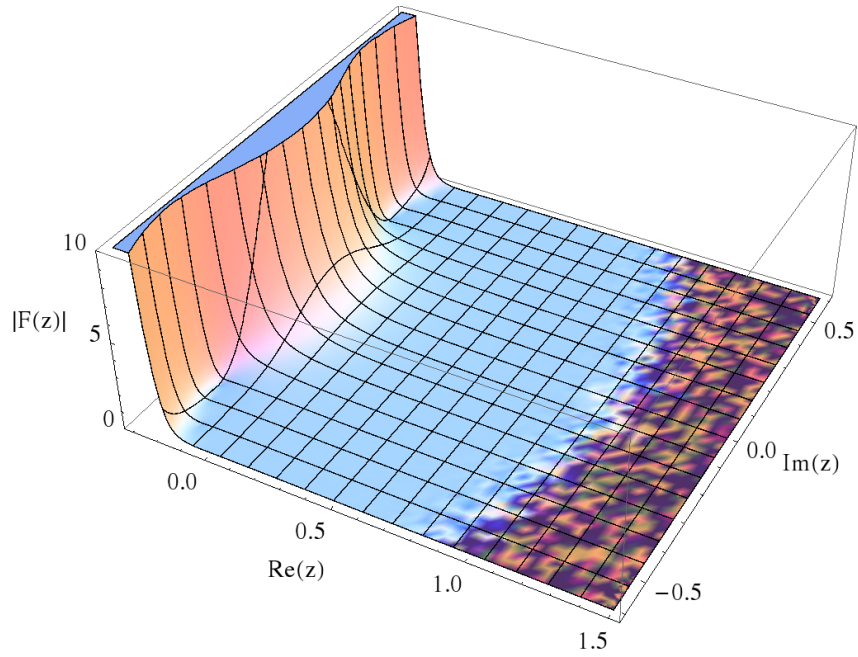
Figure 5.19.: Magnitude of the 40th Faber polynomial corresponding to the BW mapping illustrated in figure 5.14 shifted by 0.2
