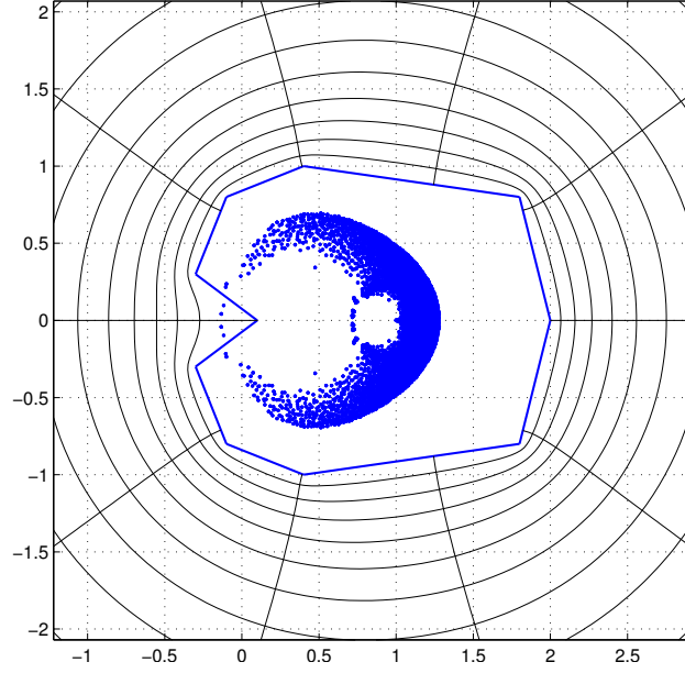
Figure 5.22.: A polygon enclosing the eigenspectrum of the mass-preconditioned D created using the SC Toolbox. The curves outside the polygon are preimages of circles of radius R outside the unit disk
