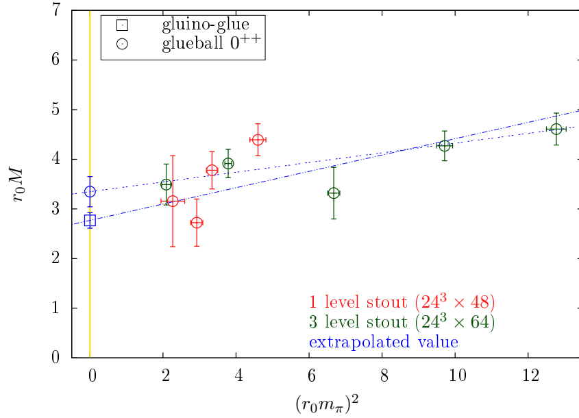
Figure 6.6.: The glueball mass as a function of the squared mass of the adjoint pion in units of the Sommer scale, the corresponding linear fit and the fit for the gluino-gluon
