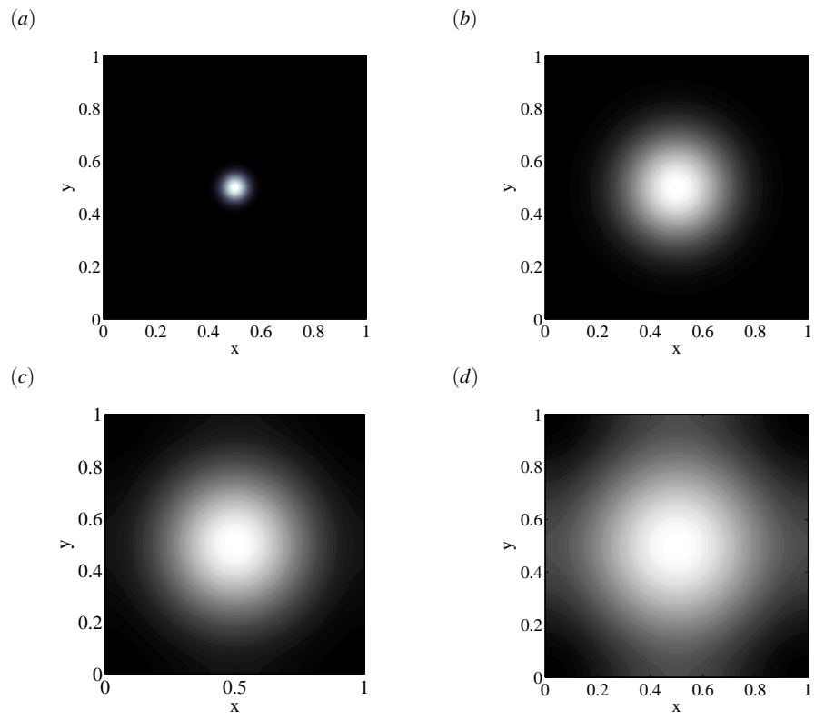
Fig. 7.9 Numerical solution of the two-dimensional diffusion equation 7.2 by means of the ADI method (7.19), calculated at four different time moments: (a) t=0 ; (b) t=10 ; (c) t=20 ; (d) t=40 .
