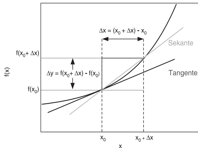
Abbildung III.7: Differenzenquotient
