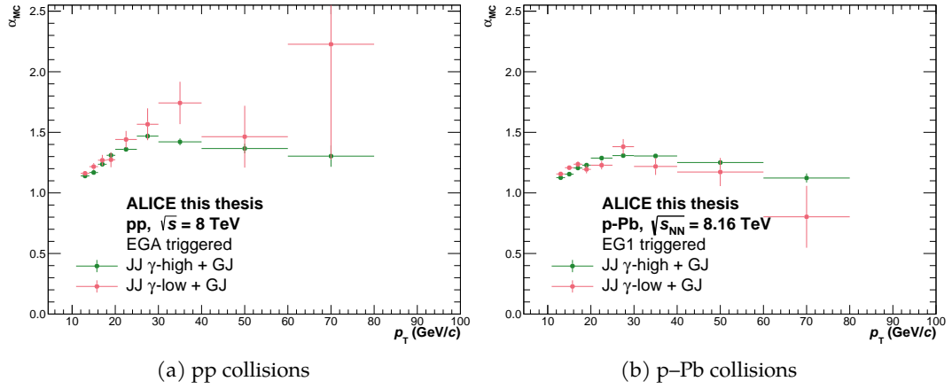
Figure 8.7: Correction factors \alpha_{MC} calculated according to Eq. 8.11 to account for the correlation of shower shape and isolation quantity. For clusters with p_T < 16 \text{ GeV}/c the factors are obtained using the sum of GJ MC and JJ \gamma -low MC , whereas the respective JJ \gamma -high production is used above this threshold.
