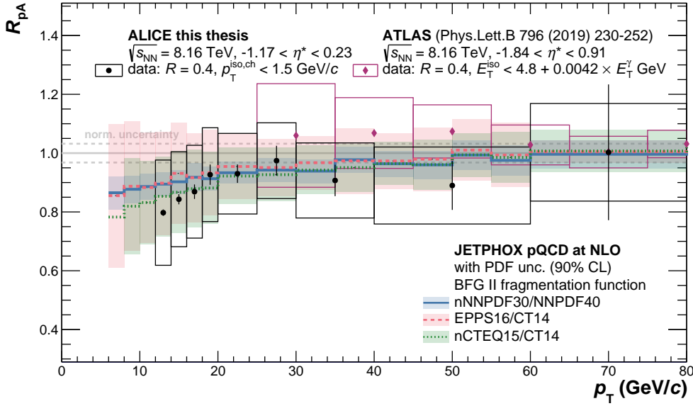
Figure 11.5: Nuclear modification factor ( R_{pA} ) of isolated prompt photon production in p–Pb collisions at \sqrt{s_{NN}} = 8.16 \text{ TeV} . The vertical error bars and boxes denote the statistical and systematic uncertainties, respectively. The dashed grey lines indicate the normalization uncertainty of 3.2 %. The measurement is compared to various pQCD calculations at NLO, where the used (n)PDFs and fragmentation function are given in the legend. The shown theory uncertainty bands are the respective nPDF uncertainties. The theory scale uncertainties were found to be fully correlated between both collision systems and are therefore negligible and not shown.
