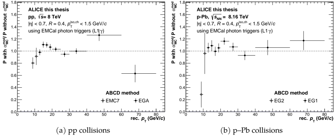
Figure 8.9: Impact of a modified correction \alpha_{MC}^{\text{mod}} given in Eq. 8.13 on the purity estimate using the ABCD method. The purity ratio with and without this additional correction is shown for the pp and p-Pb sample, respectively, where the used EMCal triggers are denoted in the legend.
