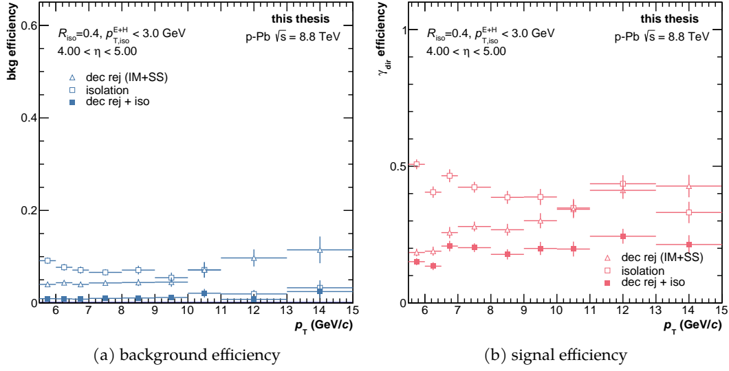
Figure A.8: Left: Reconstruction efficiency for background clusters in p-Pb collisions at \sqrt{s_{NN}} = 8.8 TeV obtained using PYTHIA6 and full detector simulation in GEANT3 for various selections, which are outlined in the text. Right: Reconstruction efficiency for signal photons in the same collision systems. A low reconstruction efficiency for the background sample and a high efficiency for the signal sample are desirable.
