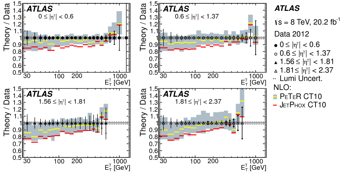
Figure 2.28: Measurement of isolated prompt photon production in pp collisions at \sqrt{s} = 8 \text{ TeV} by ATLAS [113].
