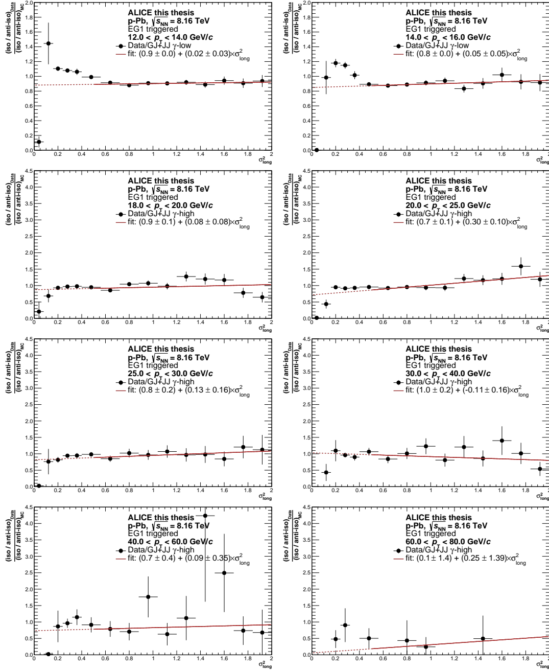
Figure A.5: Double ratio calculated according to Eq. 8.5 in various p_T -intervals for EG1 triggered p-Pb collisions at \sqrt{s_{\text{NN}}} = 8.16 TeV. A first-order polynomial fit is indicated by a red line, where the solid part of the line indicates the fit region. A slope of \approx 0 indicates agreement between data and MC in their description of the isolation dependence of the shower shape parameter.
