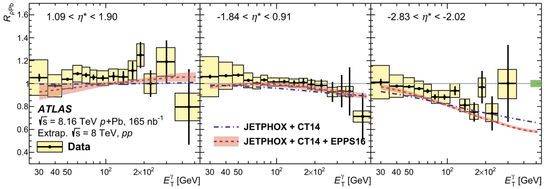
(b) Nuclear modification factor R_{pA}
