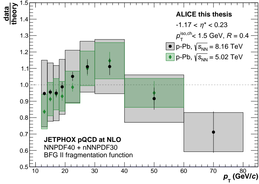
Figure 11.3: Ratio of the isolated prompt photon production cross section measurement in p–Pb collisions at \sqrt{s_{\text{NN}}} = 8.16 TeV and 5.02 TeV [241] with respect to pQCD calculations at NLO. Note: The measurement in p–Pb collisions at \sqrt{s_{\text{NN}}} = 5.02 TeV has preliminary status and is not yet part of an ALICE paper. The factor \kappa_{\text{MC}} is given in Eq. 7.7. While it is included in the signal efficiency for the measurement at \sqrt{s_{\text{NN}}} = 8.16 TeV, it is instead used as a scaling for the NLO calculation for the measurement at \sqrt{s_{\text{NN}}} = 5.02 TeV.
