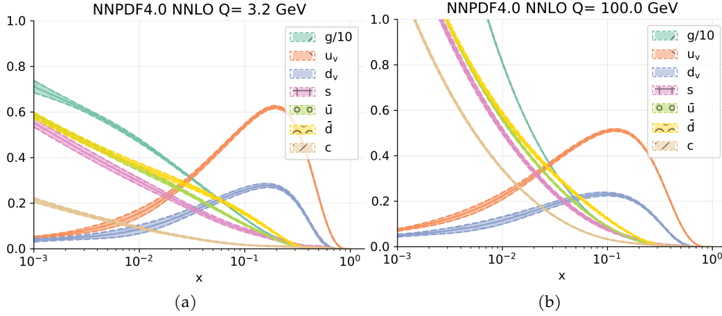
Figure 2.9: NNP4.0 NNLO proton PDF [24] as a function of momentum fraction x , evaluated at two different scales Q = 3.2 \text{ GeV} (left) and Q = 100 \text{ GeV} (right). Each colour represents the PDF of a different parton species, as indicated in the legend.
