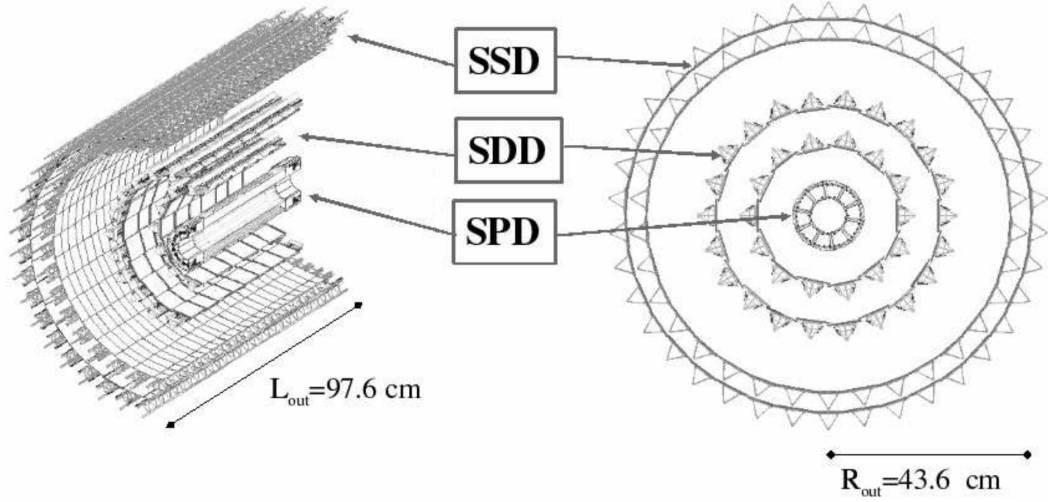
Figure 3.4: Layout of the ITS [164].
