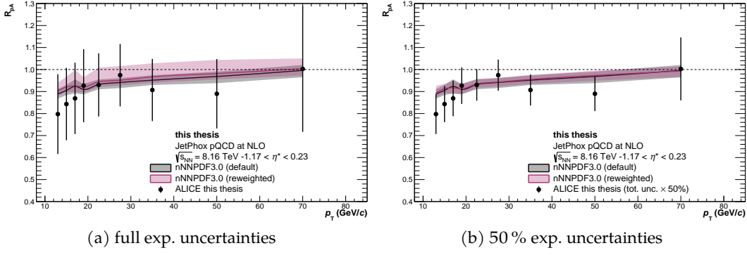
Figure 11.6: Reweighting study of potential constraints for the nNNPDF3.0 nPDF using the isolated prompt photon production R_{pA} at \sqrt{s_{NN}} = 8.16 TeV presented in this work. The ALICE data is denoted by black markers, where the vertical lines denote the total experimental uncertainties, including the normalization uncertainty added in quadrature. The right panel showcases a hypothetical scenario, where the experimental uncertainties have been reduced by a factor of 0.5. The data is shown together with JETPHOX predictions using the nNNPDF3.0 to describe the lead nucleus, where shaded bands denote the 90 % CL PDFs uncertainties. The red bands denote the uncertainty taking into account the new experimental data in a Bayesian reweighting procedure, which is outlined in the text.
