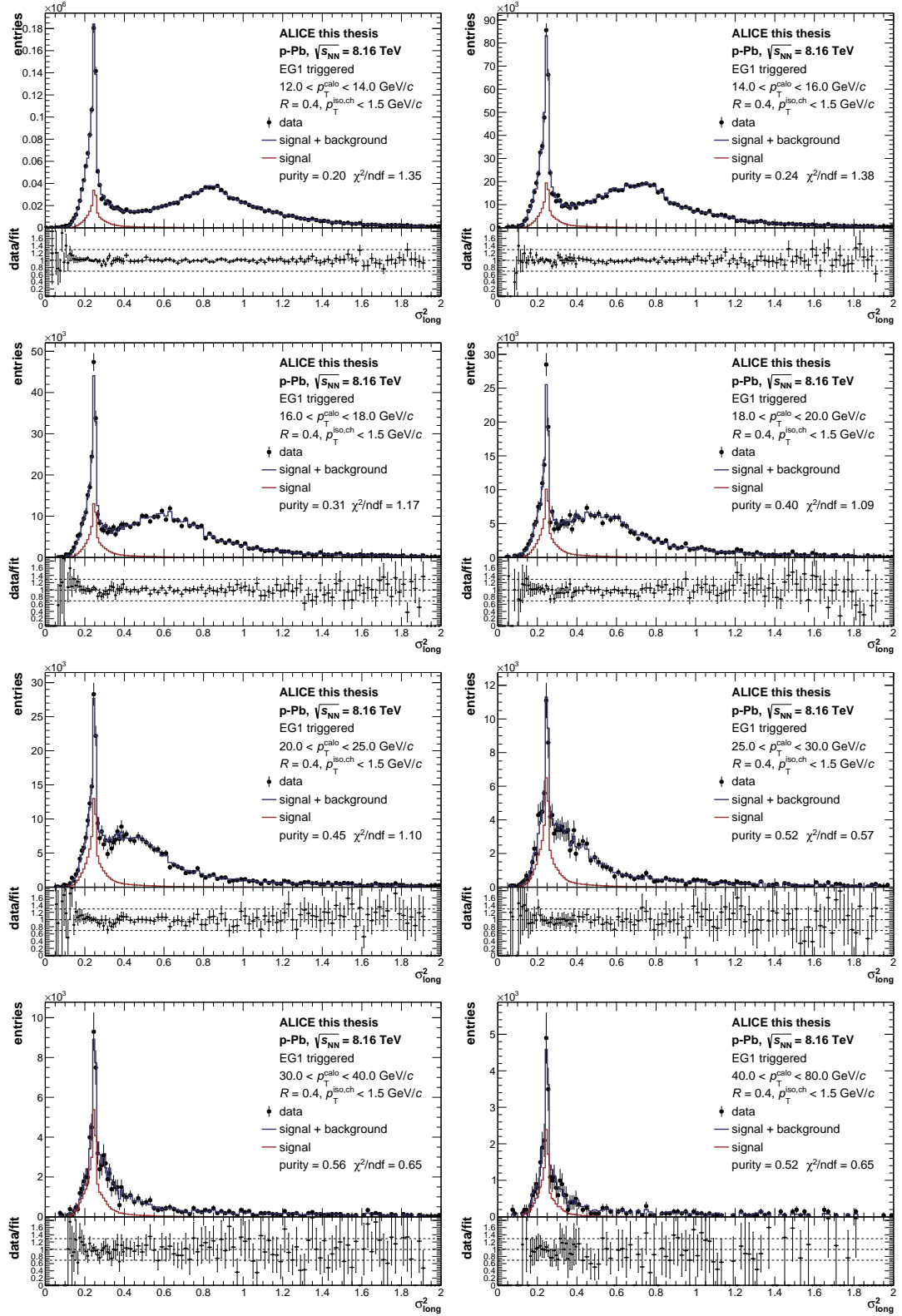
Figure 8.2: Two-component template fit (Eq. 8.2) of the long axis \sigma_{\text{long}}^2 of the shower shape ellipse in p-Pb collisions at \sqrt{s_{\text{NN}}} = 8.16 TeV for different cluster p_T intervals. The signal and background templates are obtained from GJMC and data, respectively, as outlined in the text. The purity is obtained in the photon signal region 0.1 \leq \sigma_{\text{long}}^2 \leq 0.3 according to Eq. 8.3.
