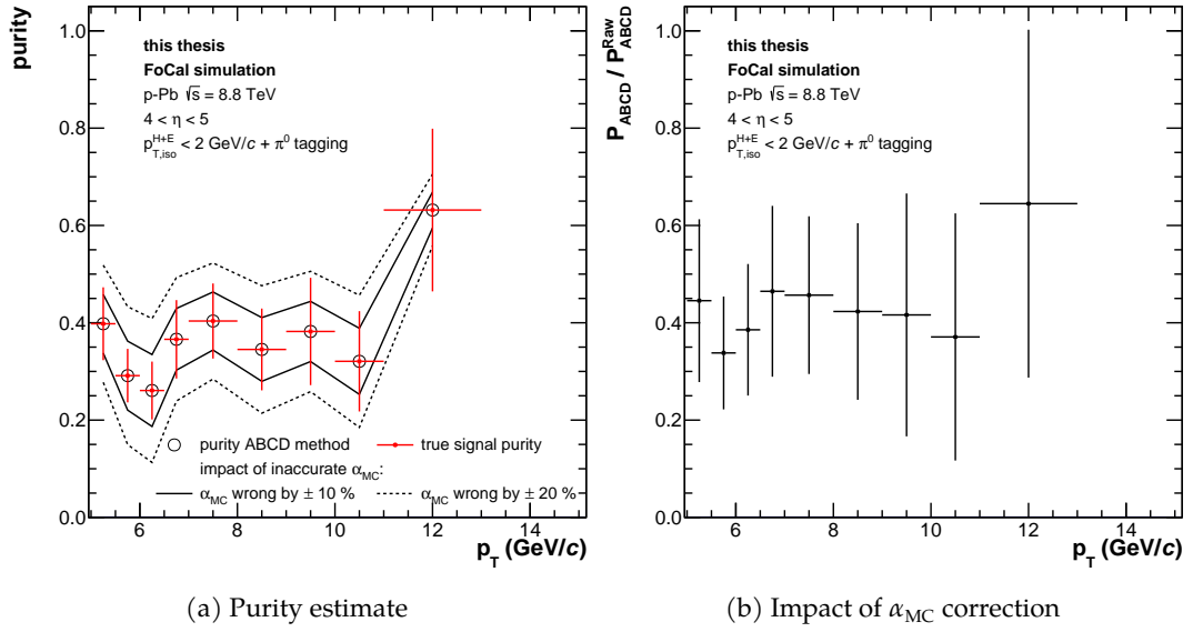
Figure A.9: Left: Isolated prompt photon signal purity for clusters measured with the FoCal within 4 < \eta < 5 in simulated p–Pb collision events at \sqrt{s_{\text{NN}}} = 8.8 TeV. A purity estimate using the ABCD method according to Eq. 8.11 (black markers) is in agreement with the true signal purity of the MB+GJ PYTHIA sample. Dashed and solid lines indicate the impact of a potential wrong determination of \alpha_{\text{MC}} on the purity estimate, which may arise if the used MCs do not accurately describe the correlation of shower shape and isolation energy in data. Right: Ratio of the purity estimate obtained with and without the aforementioned \alpha_{\text{MC}} correction.
