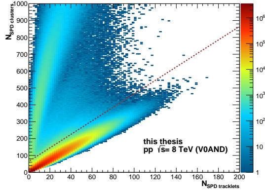
Figure 4.1: Number of SPD clusters as a function of SPD tracklets. The visible correlation can be used to suppress background events e.g. from beam-gas interactions. Events located above the red dashed line are rejected.
