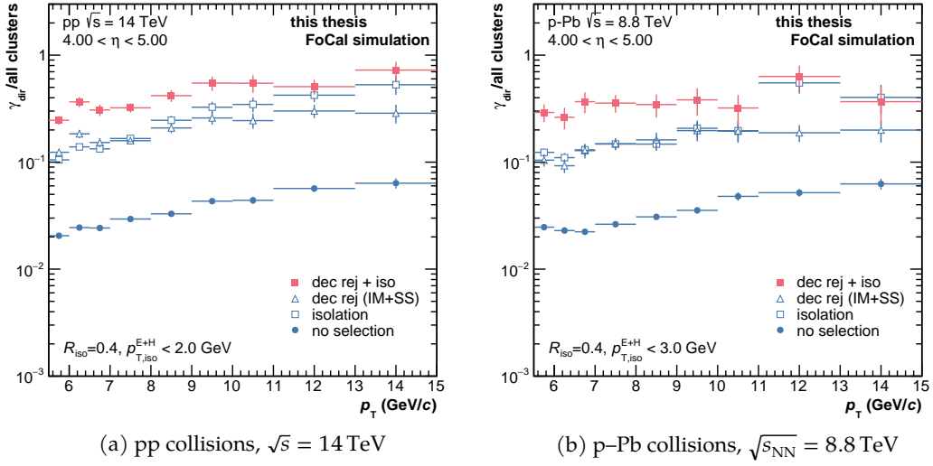
Figure 12.10: Fraction of clusters produced by direct prompt photons with respect to all clusters produced in pp and p-Pb collisions at \sqrt{s_{NN}} = 14 TeV and 8.8 TeV, respectively. The ratios are obtained using PYTHIA simulations, where MB and direct prompt photon processes are weighted with their respective cross sections. Several background rejection criteria are given in the legend, which significantly improve the fraction of direct prompt photon clusters in the sample.
