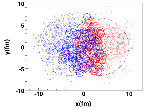
Figure 2.12: Illustration of a Pb–Pb collision with b \approx 7 fm in the picture of the Glauber model. Nucleons participating in the collision are shown as solid lines, whereas spectators are indicated by dashed lines [35].
