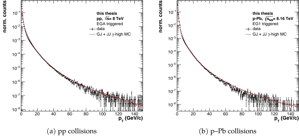
Figure 6.3: Comparison of track transverse momentum ( p_T ) reconstructed in data and the MC sample in pp (left) and p-Pb collisions (right).
