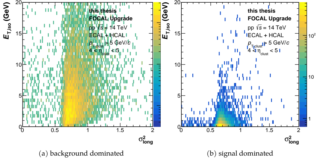
Figure 12.11: Isolation energy E_{T,\text{iso}} as a function of shower shape parameter \sigma_{\text{long}}^2 for PYTHIA MB events (left) and GJ events (right) propagated through the detector geometry using GEANT3.
