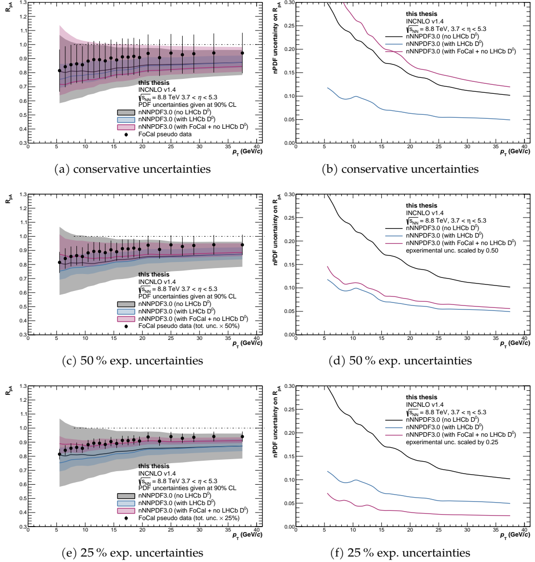
Figure 12.19: Impact of the FoCal pseudo data on nNNPDF3.0 set when excluding the LHCb measurement of D^0 meson production [130] at forward rapidities. The impact is estimated on the level of the prompt photon R_{pA} using a Bayesian reweighting of the nPDF members. The R_{pA} for each member is obtained using INCNLO calculations at NLO , and the shaded bands denote the respective nPDF uncertainty at 90% CL. The nNNPDF3.0 with A = 1 is used as the free-proton reference. Each row of figures illustrates the impact for different assumed systematic uncertainties of the pseudo data. The panels on the right show the respective relative nPDF uncertainties.
