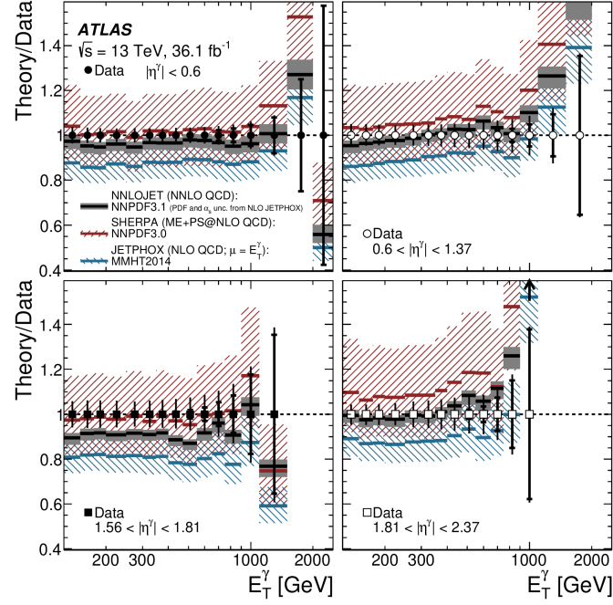
Figure 2.29: Ratio of various theoretical calculations over ATLAS data in pp collisions at \sqrt{s} = 13 TeV [91].
