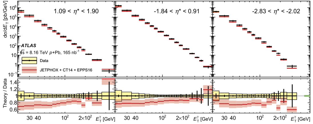
(a) Isolated prompt photon cross-section
