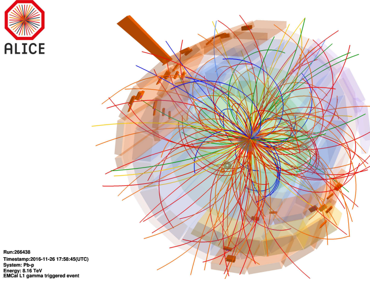
Figure 3.18: Event display of fully reconstructed exemplary p–Pb collision event at \sqrt{s_{\text{NN}}} = 8.16 TeV which was recorded using the L1 EMCal gamma trigger [209] . Reconstructed charged tracks are indicated as solid lines and energy deposits in the EMCal are represented by orange towers.
