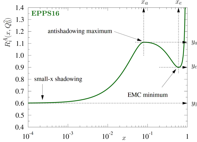
Figure 2.17: Illustration of the function used in EPPS16 [65] to describe the nuclear modification R_i^A(x, Q_0^2) of a free-proton PDF, where Q_0^2 is the parametrization scale which was set to the charm pole mass m_c = 1.3 \text{ GeV} . The different effects leading to a suppression/enhancement in different x regimes are outlined in the text.
