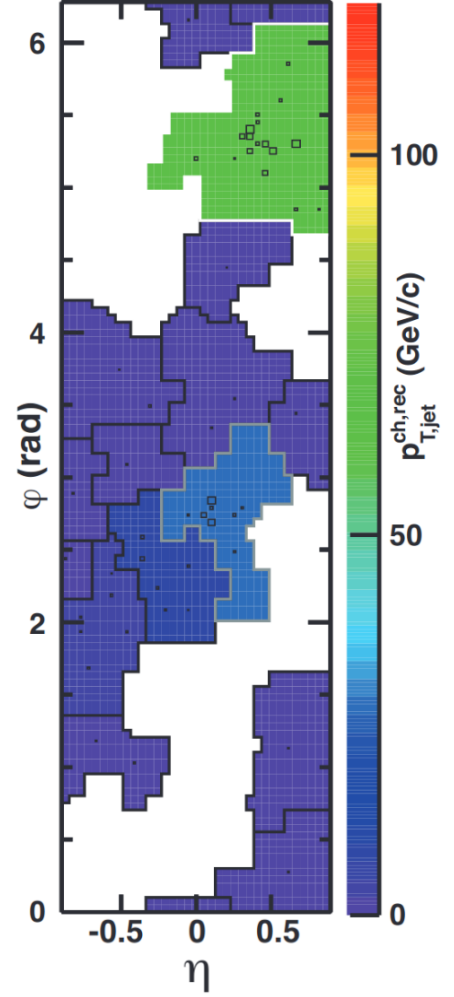
Figure 6.4: Reconstructed charged jets using the k_T algorithm shown for a pp collision at \sqrt{s} = 2.76 TeV simulated with PYTHIA. Figure adapted from Ref. [40].
