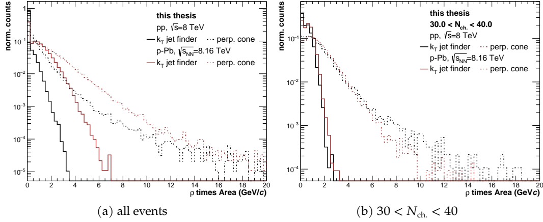
Figure 6.5: Estimates of the UE density \rho in pp and p-Pb collisions for two different estimation approaches. The densities are multiplied with the isolation cone area \pi \cdot 0.4^2 to illustrate the contribution of the UE to the charged isolation. The left figure shows the UE estimates for events fulfilling the highest available EMCal trigger in the respective collision system, whereas a selection according to the number of charged tracks N_{\text{ch}} in a given event is imposed in addition for the figure on the right.
