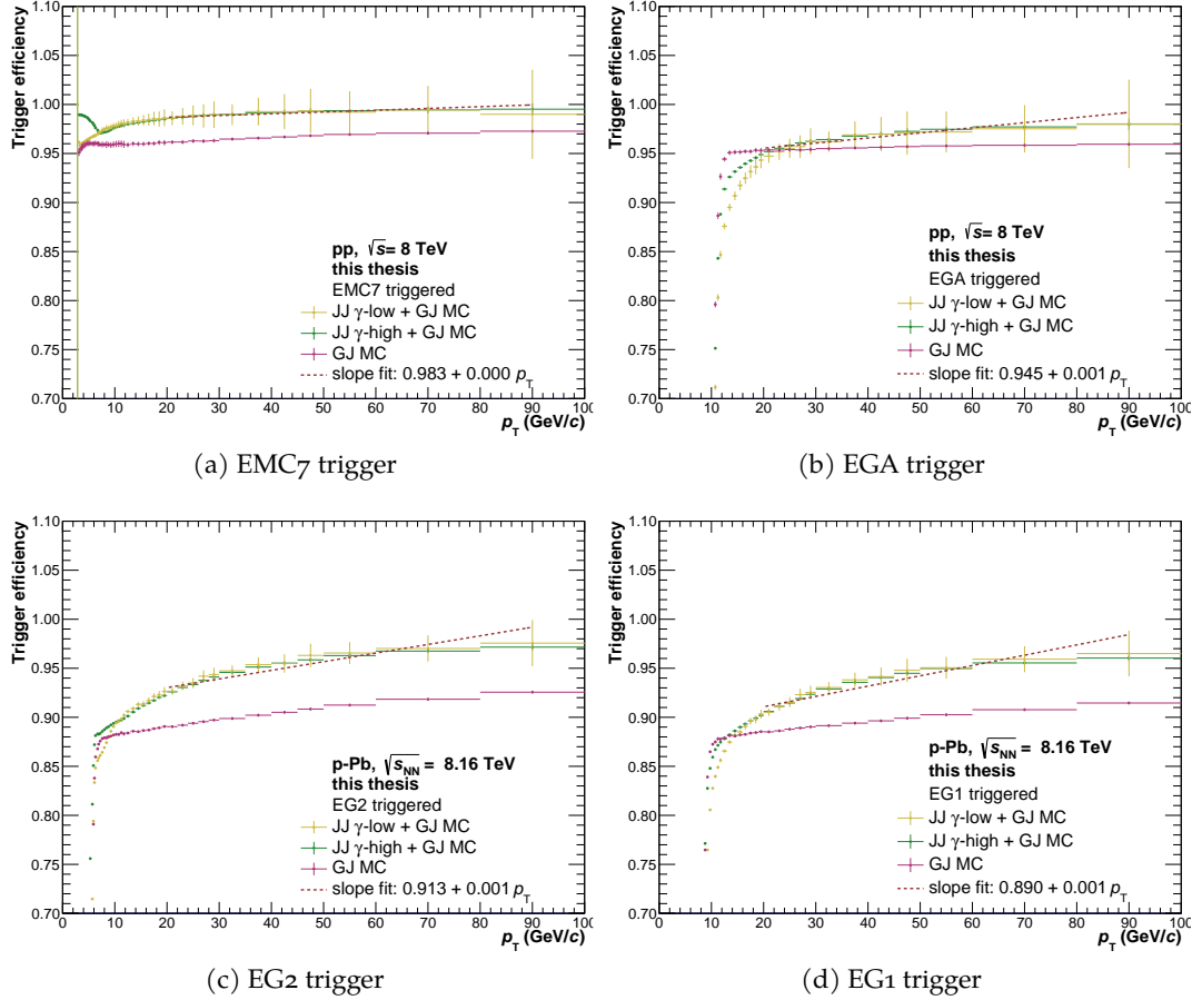
Figure 4.4: Trigger efficiencies as a function of EMCal cluster p_T for different MC samples and triggers. The samples specified as “JJ \gamma -low(high)+GJ” are obtained as the sum of the respective JJ and GJ , where weights according to the absolute cross sections obtained from PYTHIA are applied.
