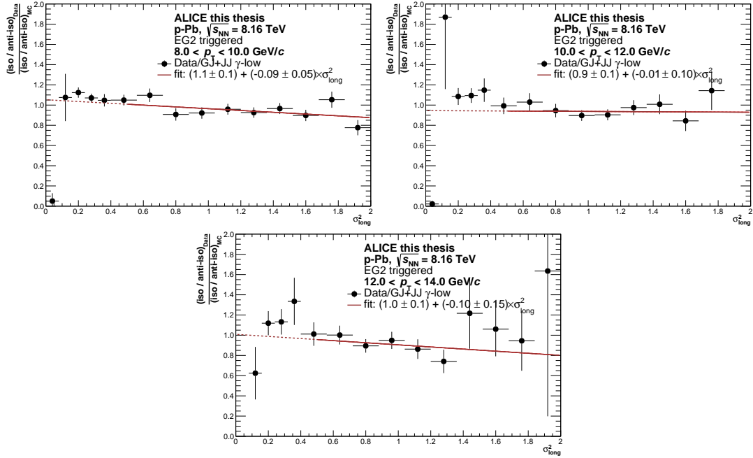
Figure A.7: Double ratio calculated according to Eq. 8.5 in various p_T -intervals for EG2 triggered p-Pb collisions at \sqrt{s_{\text{NN}}} = 8.16 TeV. A first-order polynomial fit is indicated by a red line, where the solid part of the line indicates the fit region. A slope of \approx 0 indicates agreement between data and MC in their description of the isolation dependence of the shower shape parameter.
