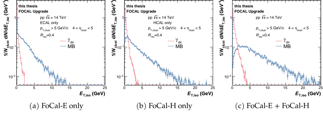
Figure 12.6: Isolation energy ( E_{T,iso} ) for all FoCal clusters with p_{T,clust} > 5 \text{ GeV} found within 4 < \eta < 5 , calculated in a cone with R = 0.4 around the given cluster. The isolation energy is calculated using the detectors given in the respective caption. The different colours indicate the processes included in the Pythia simulation of pp collisions at \sqrt{s} = 14 \text{ TeV} , resulting in a prompt photon signal dominated sample (red) and decay photon dominated sample (blue).
