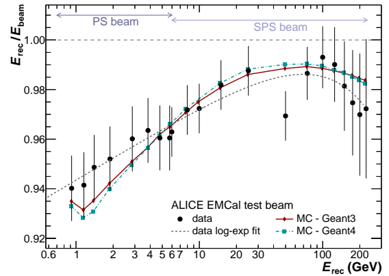
Figure 5.3: Energy response of the EMCal calorimeter to electrons obtained using a test beam setup [227] at the PS and SPS. Figure taken from Ref. [184].
