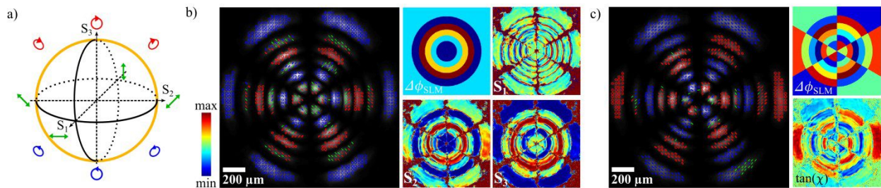
Figure 7. Poincaré beams: even Laguerre-Gaussian beams ( LG_{5,3}^e ) with spatially varying states of polarization. The reachable states of polarization for the used setting \beta_1 = -45^\circ and \beta_2 = 90^\circ are depicted on the Poincaré sphere in a). b) shows the measured transverse plane of a Laguerre-Gaussian beam, while each intensity ring has its own state of polarization (red/ blue: right/ left elliptical states of polarization, green: linear states of polarization). The LG_{5,3}^e -beam is generated by the first half of the SLM (amplitude and phase modulation), while the SPM creates the desired distribution of polarization by the use of the phase hologram \Delta\phi_{\text{SLM}} (min = 0, max = 2\pi ) illustrated in the subfigure. The measured Stokes parameters S_1 , S_2 and S_3 (min = -1, max = 1) match the modulated ring structure. Subfigure c) also shows a modulated LG_{5,3}^e -beam, while in this case each intensity spot in the transverse plane has its own state of polarization as additionally visible in the corresponding polarization modulation hologram \Delta\phi_{\text{SLM}} and the measured opening angle of polarization ellipses ( \tan(\chi) ; min = -1, max = 1).
