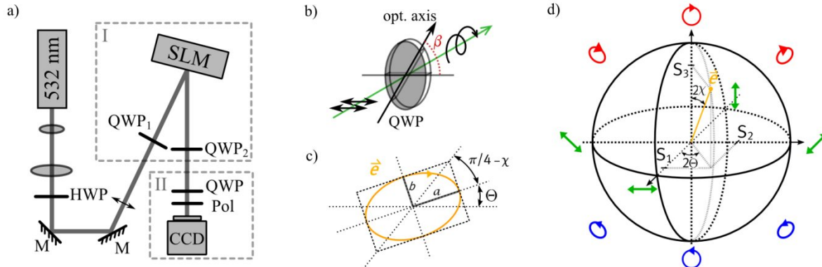
Figure 4. Spatial modulation of polarization. a) shows the outline of the experimental setup for the polarization modulation – I: spatial polarization modulator (SPM) consisting of two quarter wave plates (QWP) enclosing a spatial light modulator (SLM), II: polarization measurement setup composed of a rotatable quarter wave plate and a polarizer (Pol) in front of a CCD camera (CCD). The input polarization supposed to be modulated by the SPM is horizontally linear and created by a half wave plate (HWP). The angles of the SPM’s QWPs are chosen to be \beta_1 = -45^\circ and \beta_2 = 90^\circ regarding the input polarization (see b)), while the phase shift \Delta\phi_{\text{SLM}} introduced by the SLM is variable. Subfigure c) illustrates the parameters of the polarization ellipses and d) demonstrate the Poincaré sphere spanned by the Stokes parameters S_1 , S_2 and S_3 and used to visualize states of polarization, e.g. \vec{e} . Right/ left elliptical states of polarization are indicated as red/ blue ellipses, while linearly polarized states are colored green.
