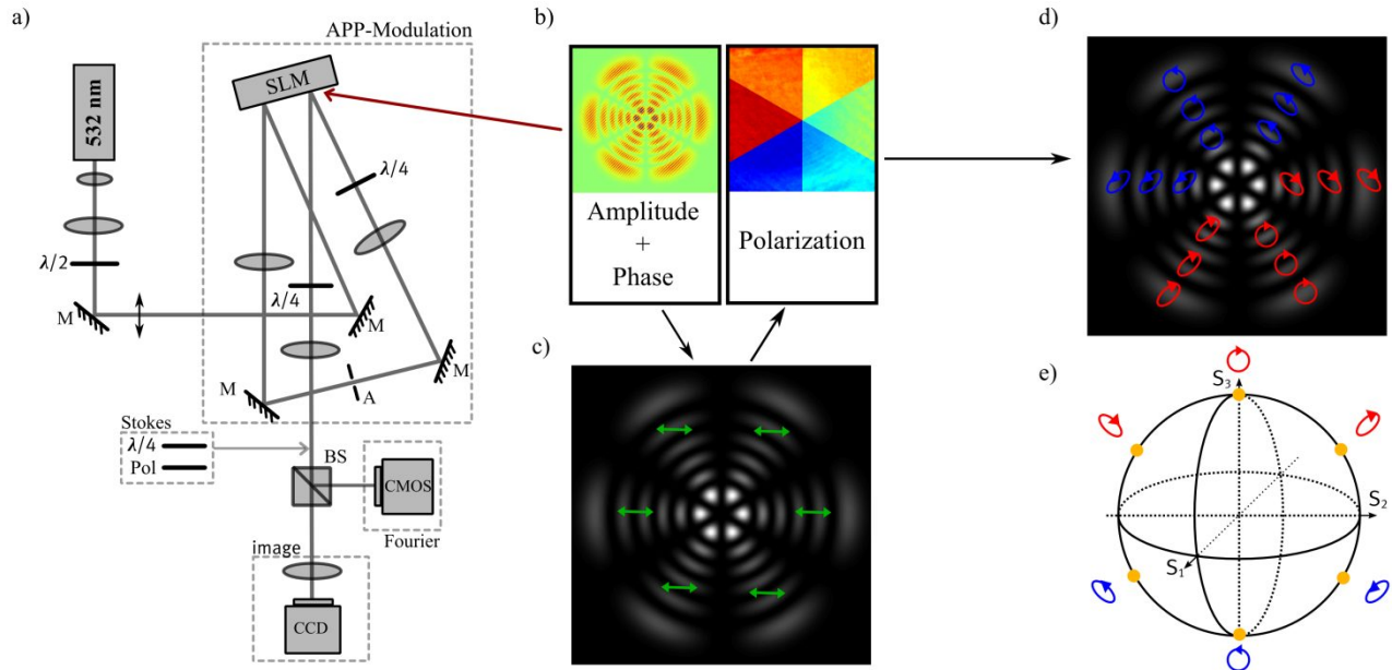
Figure 6. Outline of the experimental setup and method used for amplitude, phase and polarization modulation (APP-Modulation): the reflective, phase-only SLM is used in split-scene-mode, so that the first half can be utilized to modulate amplitude and phase (see sec. 2), the second half enclosed by two quarter wave plates ( \lambda/4 ) creates the desired polarization distribution by acting as a SPM (see sec. 3), as indicated in b) - d). b) shows the used modulation holograms including the correction holograms, while c) indicates the light field achieved after the first half of the SLM – in the shown case an even Laguerre-Gaussian beam ( LG_{5,3}^e ; grayscale image of the simulated intensity distribution is shown in the background) containing only horizontally linear polarized states (green arrows). After passing the SPM a complex light field modulated in amplitude, phase and polarization is realized as depicted in d): each wing of the LG_{5,3}^e -beam got its own state of polarization (red/ blue ellipses indicating right/ left elliptical polarization states). In e) the chosen states for the polarization modulation are shown on the Poincaré sphere. In order to determine the states of polarization, a measurement system consisting of a rotatable quarter wave plate and a polarizer (Pol) can be included into the setup, while the complex light field can be observed in the image or the Fourier plane of the SLM. ( \lambda/2 : half wave plate, M: mirror, A: aperture, BS: beam splitter, CCD/ CMOS: CCD/ CMOS camera)
