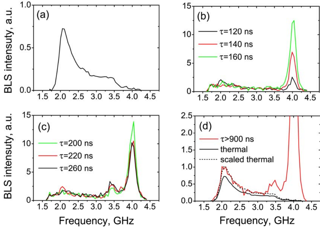
Figure 14. Evolution of the magnon frequency distribution for pumping power P_p=52 mW. (a) the BLS spectrum of thermal magnons, measured without pumping; (b), (c) magnon spectra recorded at different delays after the start of the pumping; (d) steady state distribution of magnons which is settled in the system.
