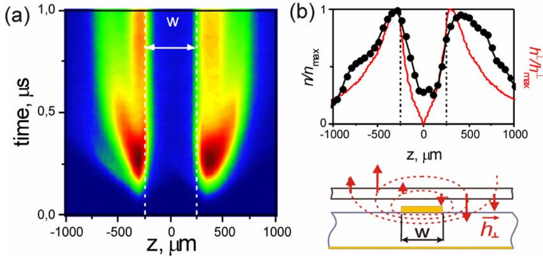
Figure 23. (a) Experimentally measured distribution of the spatial density of the condensate as a function of time in colour-coded representation for the case of microstrip resonator; static magnetic field H_0=1000 Oe, pumping power P_p=4 W. (b) Top: settled distribution of the spatial density of the condensate measured at the time delay \tau=1 \mu s and the calculated dependence of the parallel component of the pumping field h_{||}(z) ; bottom: schematic layout of the cross-section of the experimental structure.
