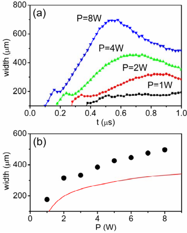
Figure 24. (a) Temporal dependences of the spatial width of the condensate clouds for the case of the two-condensate regime for different pumping powers P , as indicated. (b) Width of the condensate clouds corresponding to the end of the pumping pulse as a function of the pumping power. Points – experiment, line – theory.
