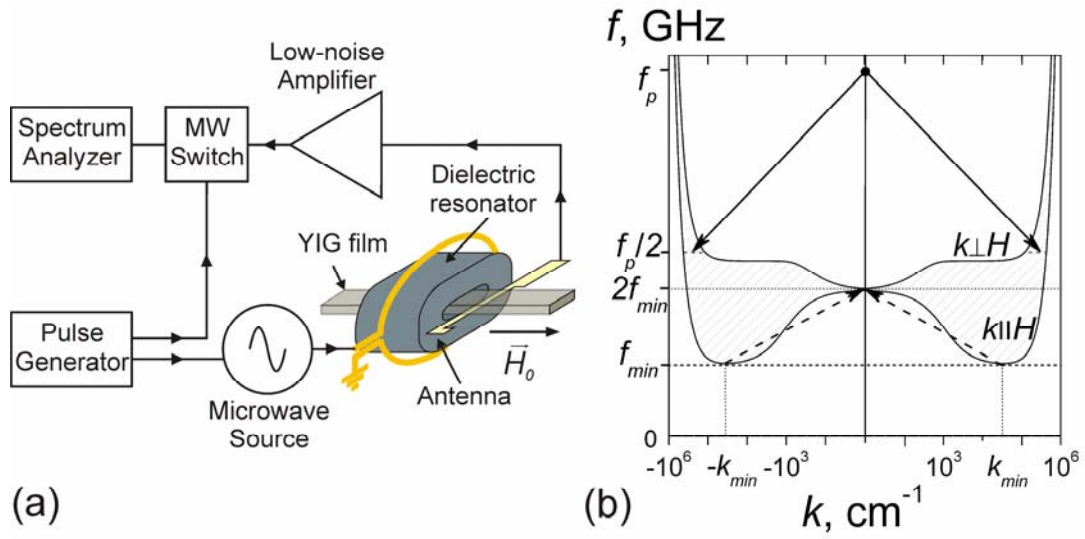
Figure 25. (a) Schematic layout of the experimental setup. (b) Spectrum of magnons for 5 \mu\text{m} thick YIG film at H_0=520 Oe. Solid lines illustrate parametric pumping process, dashed lines – confluence process of two magnons from the bottom of the spectrum.
