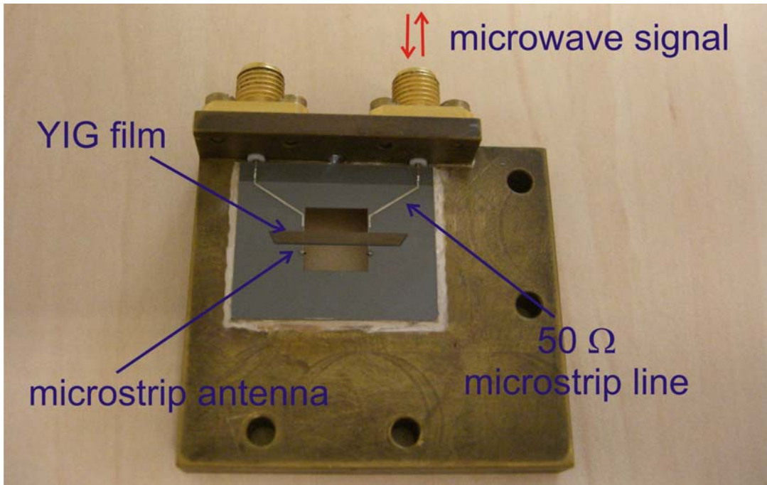
Figure 7. Conventional structure with a planar microstrip antenna used for the excitation and detection of spin waves in ferromagnetic films.
