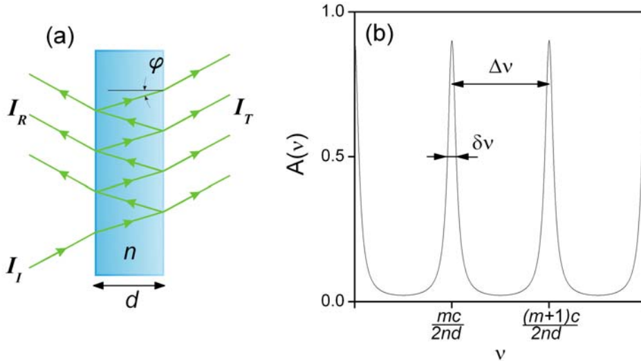
Figure 10. Schematics of the simplest Fabry-Perot interferometer (a) along with its transmission function (b).
