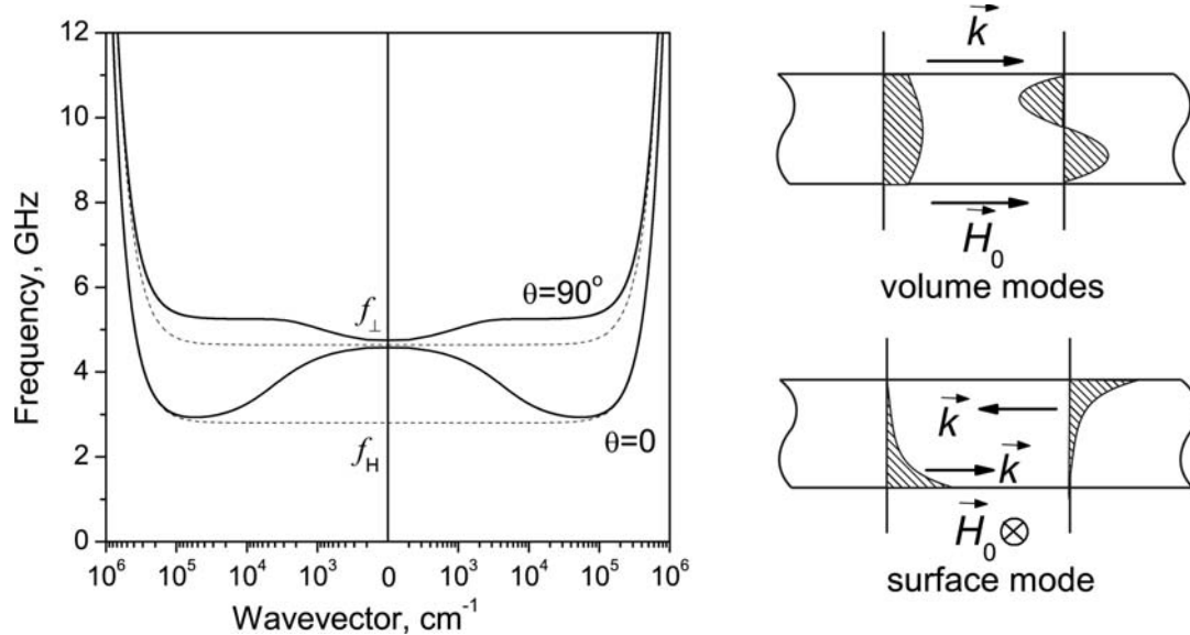
Figure 4. Spectrum of the spin waves in 5 \mu\text{m} thick in-plane magnetized YIG film at H_0=1 kOe (solid lines) along with the spectrum of the bulk ferromagnet (dotted lines) (a); (b) – schematics of the profiles of the volume and surface magnetostatic modes.
