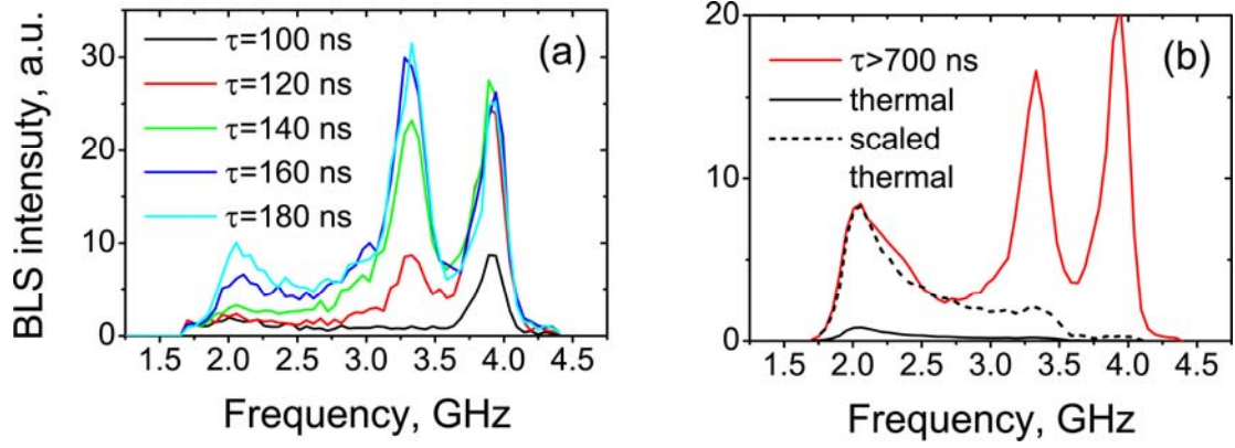
Figure 15. Time evolution of magnon distribution for pumping power P_p=171 mW
