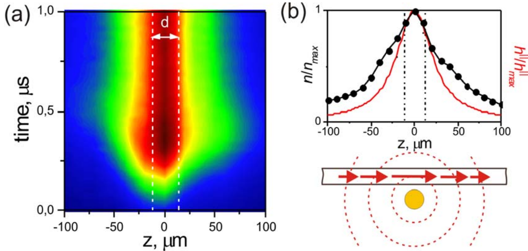
Figure 22. (a) Experimentally measured distribution of the condensate density as a function of time and distance from the centre of wire resonator in colour-coded representation; static magnetic field H_0=1000 Oe, pumping power P_p=4 W. (b) Top: settled distribution of the spatial density of the condensate measured at the time delay \tau=1 \mu\text{s} and the calculated dependence of the parallel component of the pumping field h_{||}(z) ; bottom: schematic layout of the cross-section of the experimental structure.
