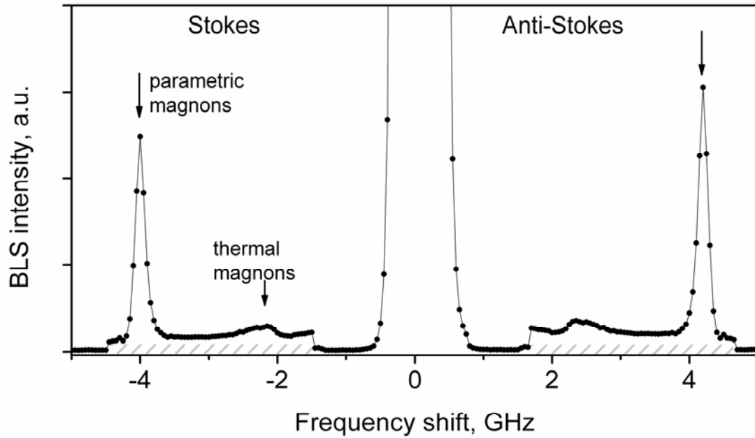
Figure 13. Experimental BLS spectrum obtained in back scattering on 5 \mu\text{m} thick tangentially magnetized YIG film under continuous excitation by parametric pumping of frequency f_p=8.1 GHz. Static magnetic field H_0=700 Oe, pumping power P_p=17 mW
