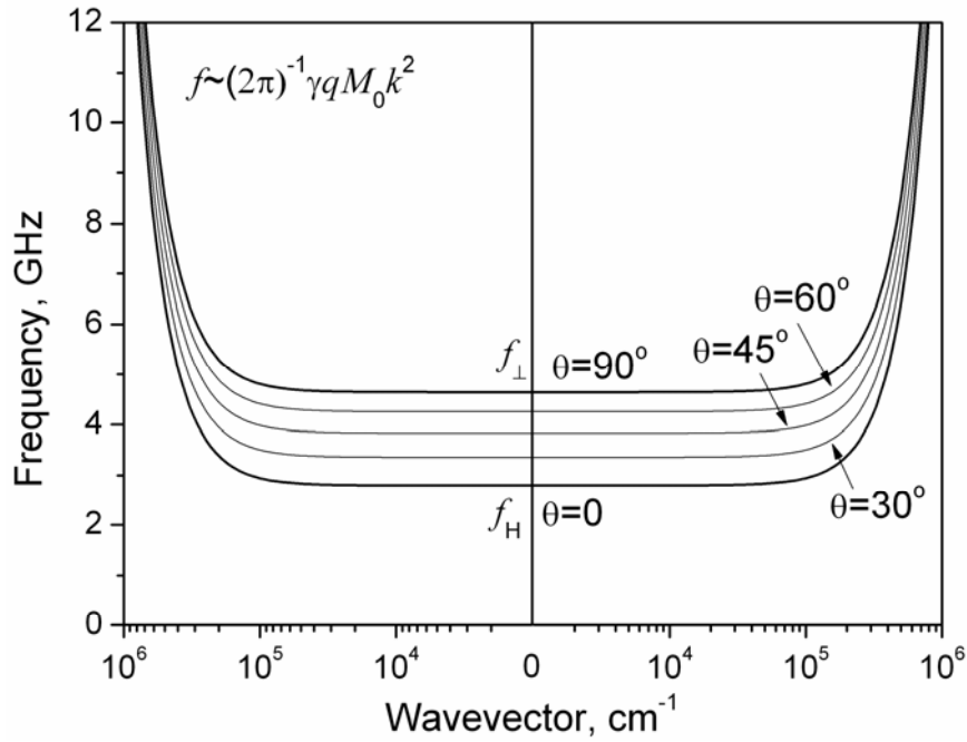
Figure 2. Spectrum of spin waves in an unbounded ferromagnet with 4\pi M_0=1750 G and q=3\times 10^{-12} cm 2 (YIG at room temperature) for H_0=1 kOe.
