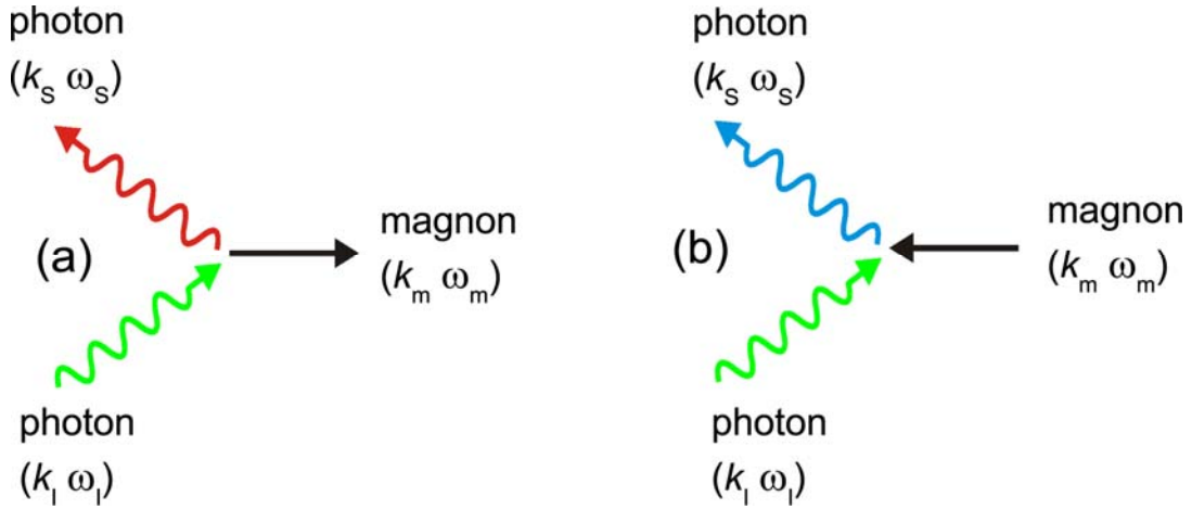
Figure 6. Illustration of Brillouin scattering process; panels (a), (b) corresponds to the Stokes ((k_s, \omega_s) = (k_l - k_m, \omega_l - \omega_m)) and anti-Stokes ((k_s, \omega_s) = (k_l + k_m, \omega_l + \omega_m)) frequency shift respectively.
