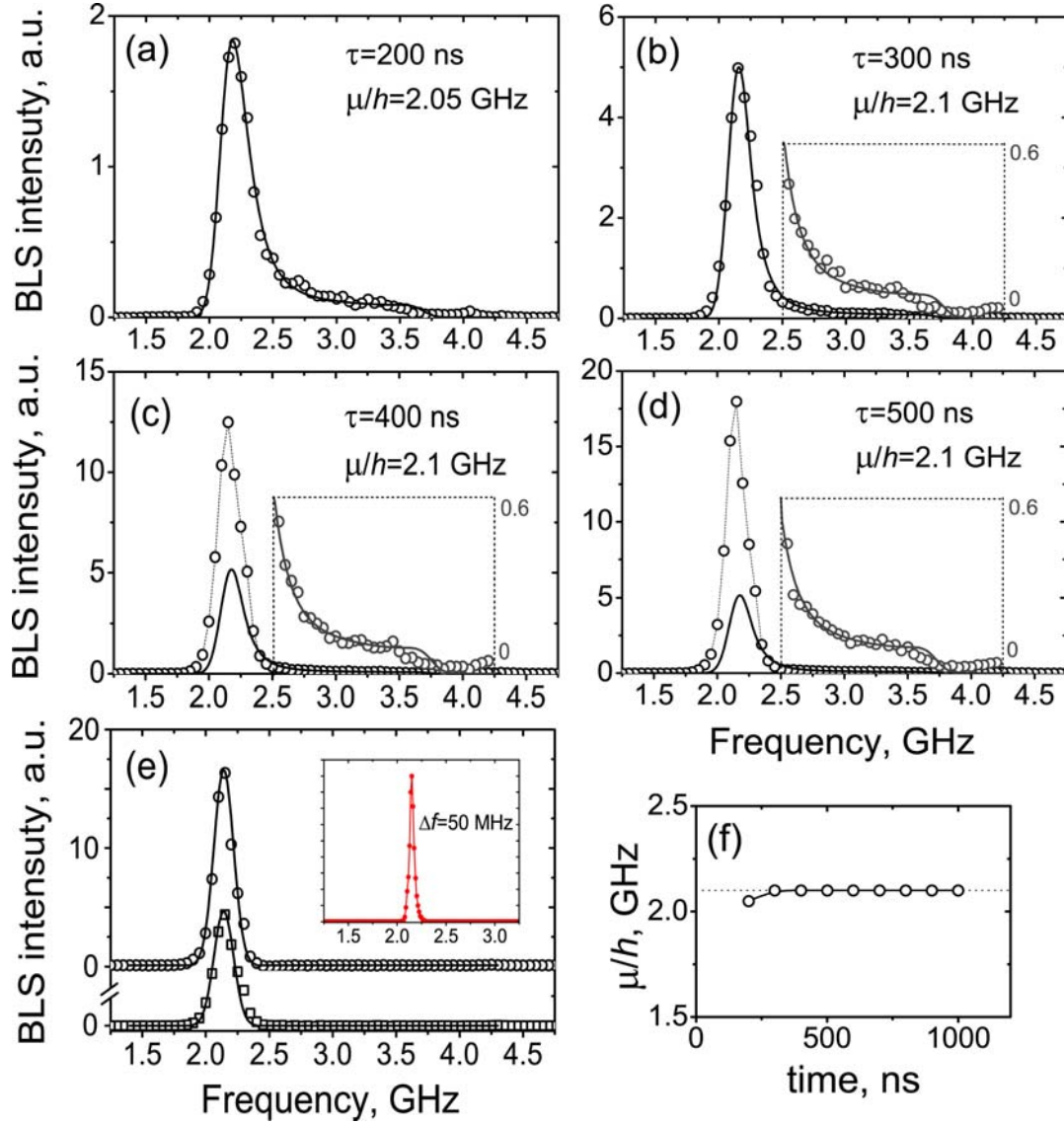
Figure 20. (a)-(d) Time evolution of magnons BLS spectrum for pumping power P_p=5.9 W: circles – experiment, solid lines in (a), (b) best fit using Eq. (20), lines in (c), (d) –calculated critical magnon distribution with \mu=\hbar f_{\min} . (e) Differences between spectra measured at \tau=400 ns and \tau=500 ns (squares and circles) and critical magnon distribution; lines – results of fit with the instrumental function of the interferometer; inset – magnon distribution measured with the ultimate resolution of the interferometer. (f) Dependence of the chemical potential of magnon gas on time.
