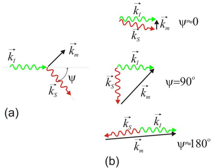
Figure 9. Kinematics of scattering process (a) – determination of the scattering angle; (b) types of scattering geometries
