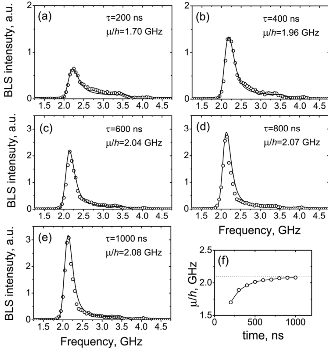
Figure 19. (a)-(e) BLS spectra of pumped magnons recorded for different delay times after the start of the pumping pulse ( P_p=4 W, H_0=700 Oe): circles – experiment, solid lines – result of the fit based on Eq. (70); (f) dependence of the chemical potential of magnon gas on time.
