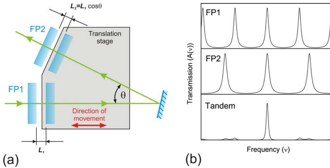
Figure 11. The arrangement (a) and the principle of operation (b) of tandem interferometer.
