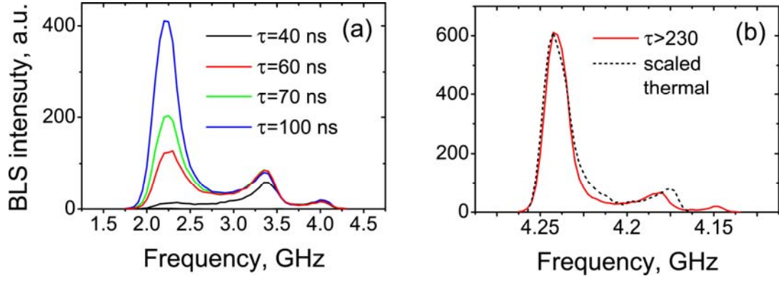
Figure 16. Time evolution of magnon distribution for pumping power P_p=0.7 W.
