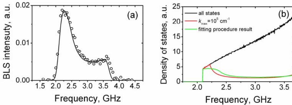
Figure 18. (a) Spectrum of thermal magnons at H_0=700 Oe: circles – experiment, solid line – fit, using Eq. (70). (b) Magnons density of states in the frequency range (f_{\min}, f_{\perp}) : black line – calculation using dispersion relation (20) with accounting for all states; red line – density of states with k < 10^5 \text{ cm}^{-1} ; green line - result of best fit optimization procedure.
