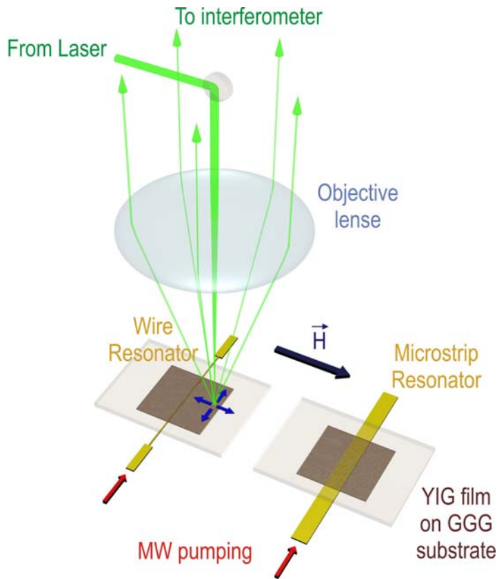
Figure 21. Arrangement of the film, pumping resonators and the probing light, used in the experiment
