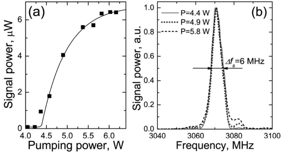
Figure 26. (a) Dependence of the power of microwave radiation vs pumping power. (b) Normalized spectra of the radiation for different pumping powers. H_0=520 \text{ Oe} .
