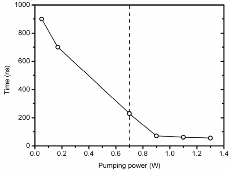
Figure 17. Time, corresponding to the appearance of a characteristic state of the magnon spectrum, as a function of pumping power. For low powers, corresponding to the left half of the graph characteristic state is described by the flow equilibrium between the pumping and the spin-lattice relaxation processes, whereas for the right one, characteristic time is the thermalization time.
