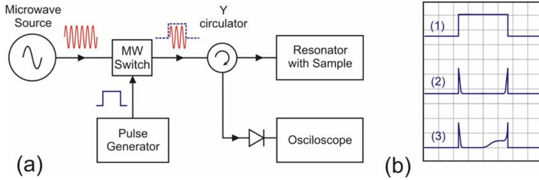
Figure 8. (a) Typical experimental setup for the parametric excitation of spin waves. (b) Oscillograms of microwave pulses: (1) incident pulse; (2) pulse, reflected from resonator below the threshold of parametric excitation; (3) reflected pulse, above the threshold.
