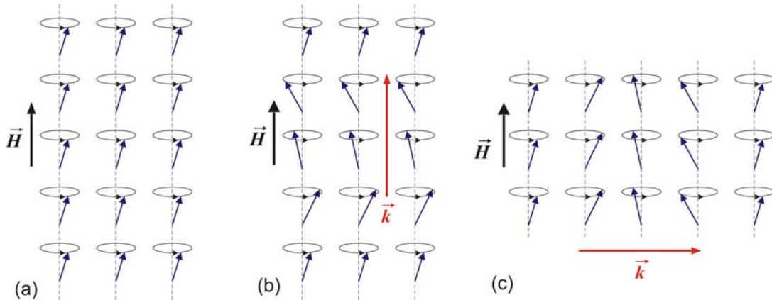
Figure 3. Schematic illustration of (a) the uniform mode and spin waves propagating along the direction of the static magnetic field (b) and perpendicularly to it (c).
