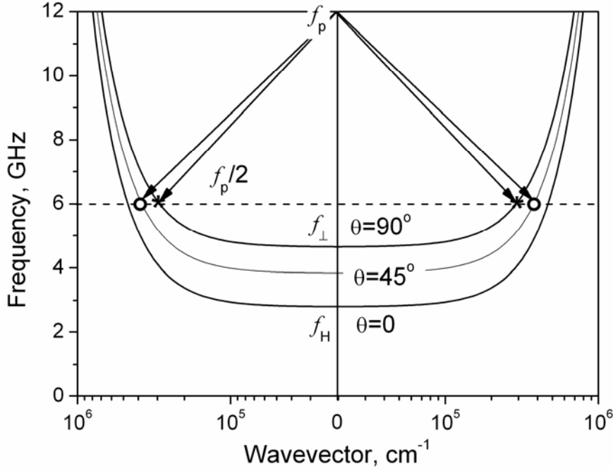
Figure 5. Illustration of the parametric pumping instability process. Circles and stars indicate the waves, which first become unstable under the influence of the perpendicular and parallel pumping respectively.
