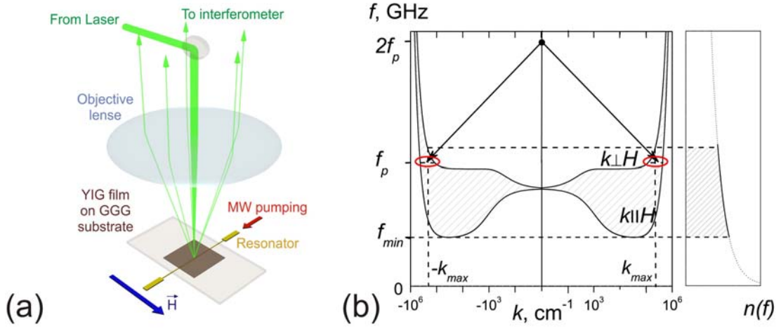
Figure 13. (a) The arrangement of the film, pumping resonators and the probing light, used in the experiment (b) The low-frequency part of the magnon spectrum in tangentially magnetized 5 \mu\text{m} thick YIG film at H_0=700 Oe. Arrows illustrate the pumping process. Right panel explains the limitations on the accessible frequencies range.
