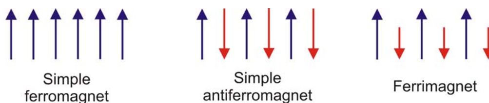
Figure 1. Arrangement of electron spins in magnetically ordered crystals
