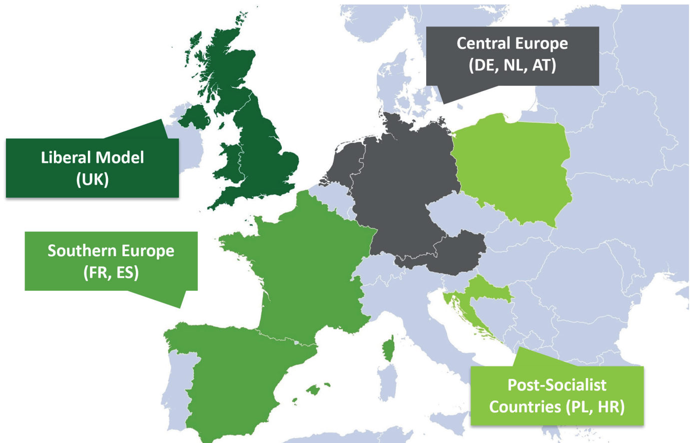
Graph 1: TSI Countries
