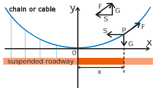
Fig. 9: A parabola emerges as a curve form for the main cable of a suspension bridge.
