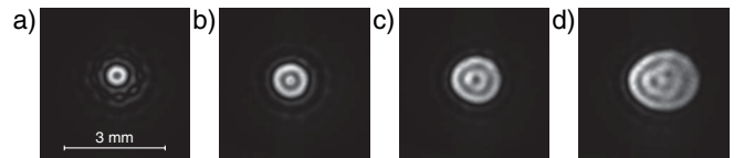
FIG. 3. Experimentally observed solitons. Parameters as in Fig. 2 with the exception of the replacements T = 327.3^\circ\text{C} , \Delta = 14.6 GHz, P_{\text{las}} = 165 mW, \Phi = 7^\circ 00' in (b) to (d).
