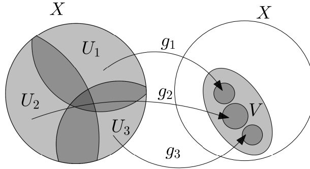
FIGURE 1. X \prec V
