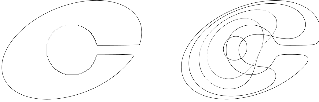
Figure 5: An original curve (left), and its evolution for times t = 1, 30, 70, 100, 140 (right).
