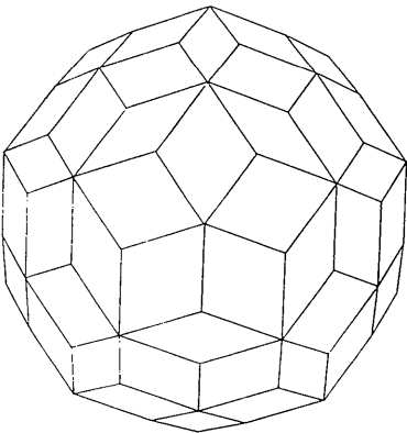
Fig. 4. (0, 10), ()(1\ 2\ 3\ 4\ 5\ 6\ 7\ 8\ 9\ 10)^\dagger, A(5) . The figure represents a rhombic enneaahedron constructed from two rhombi.
