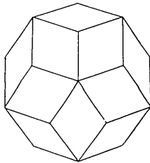
Fig. 2. (0,6), ()(1\ 2\ 3\ 4\ 5\ 6)^\dagger, A(5) . The entries, as for each of the following figures, correspond to the entries in Table 1 and are respectively (p, n - p) , the orbit representative of X_p^n and the stability group S_p^n . The dagger sign ^\dagger designates which of the stars, i.e. p -star or (n - p) -star, is used in obtaining the polyhedron figure. The figure represents the rhombic triacontahedron. Because of the angle of perspective, five faces of the front half of the figure are hidden.
