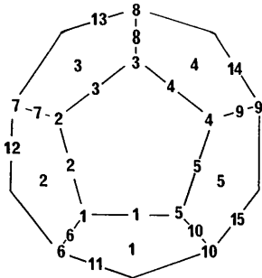
Fig. 1. The enumeration of the fivefold, threefold and twofold axes of rotation of a dodecahedron oriented face first.
