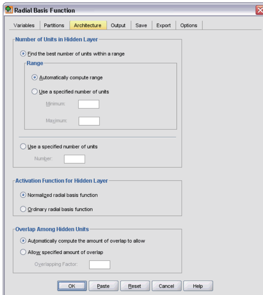
Figure 3-3 Radial Basis Function: Architecture tab
