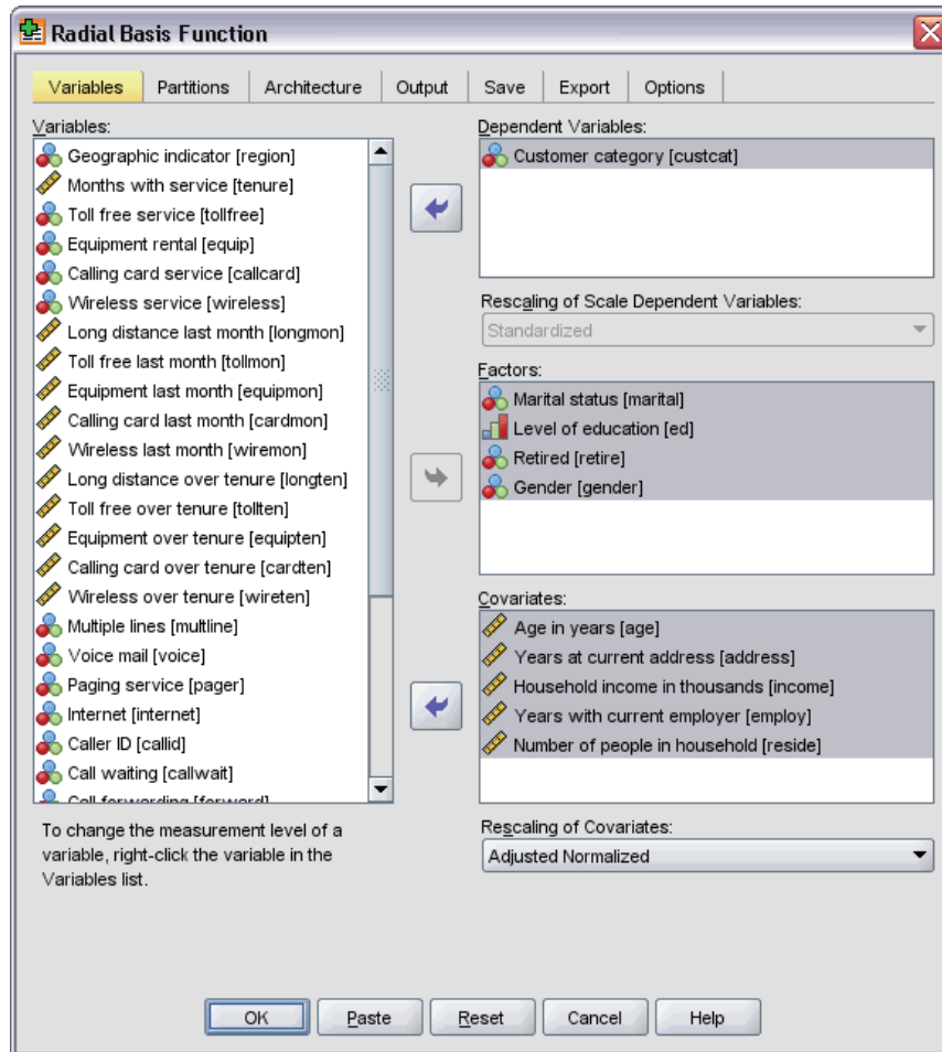
Figure 3-1 Radial Basis Function: Variables tab
