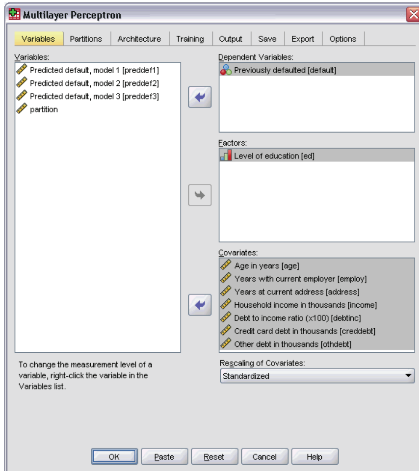
Figure 4-3 Multilayer Perceptron: Variables tab
