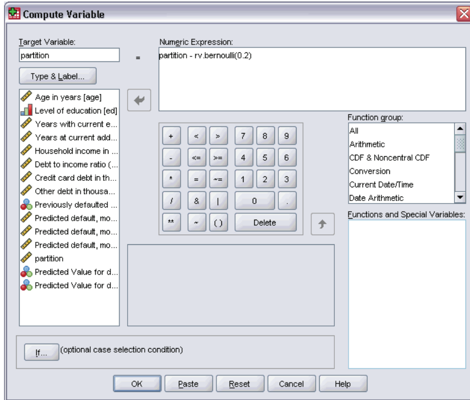
Figure 4-10 Compute Variable dialog box
