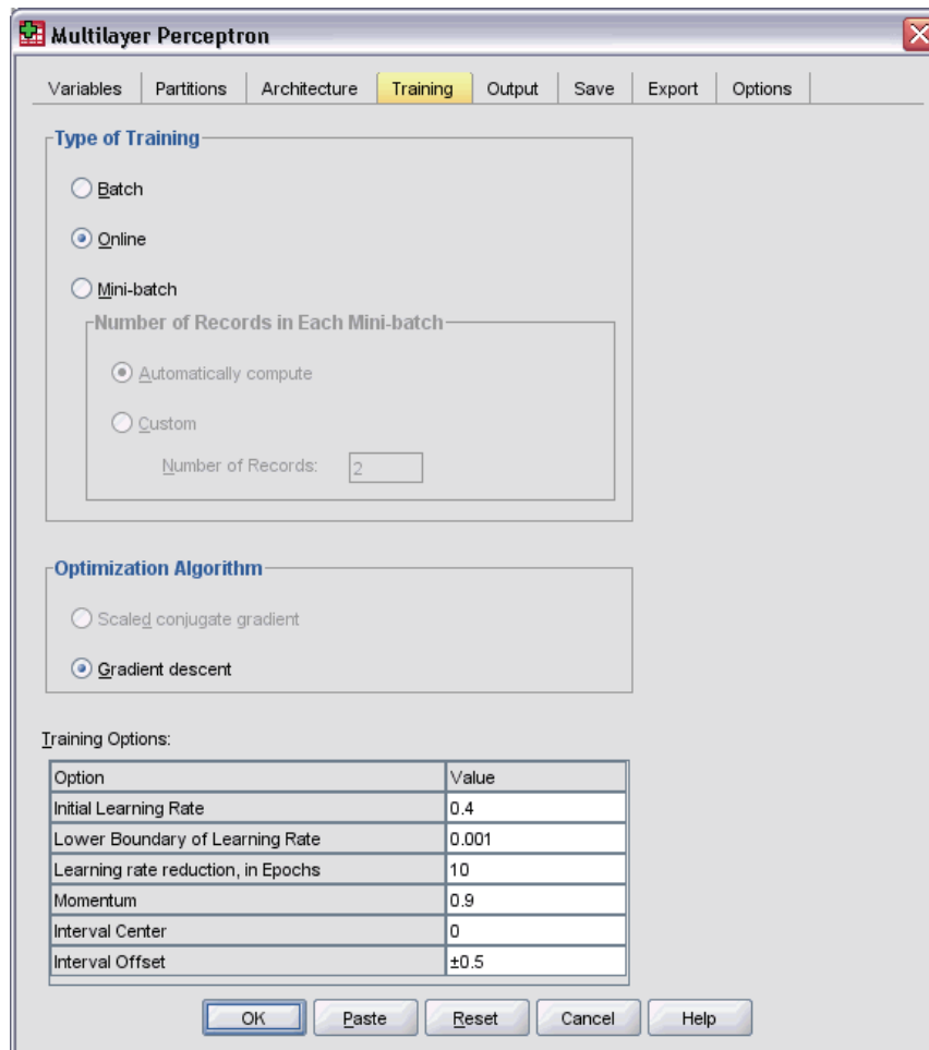
Figure 4-28 Multilayer Perceptron: Training tab
