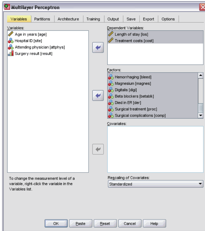
Figure 4-25 Multilayer Perceptron: Variables tab and context menu for Length of stay
