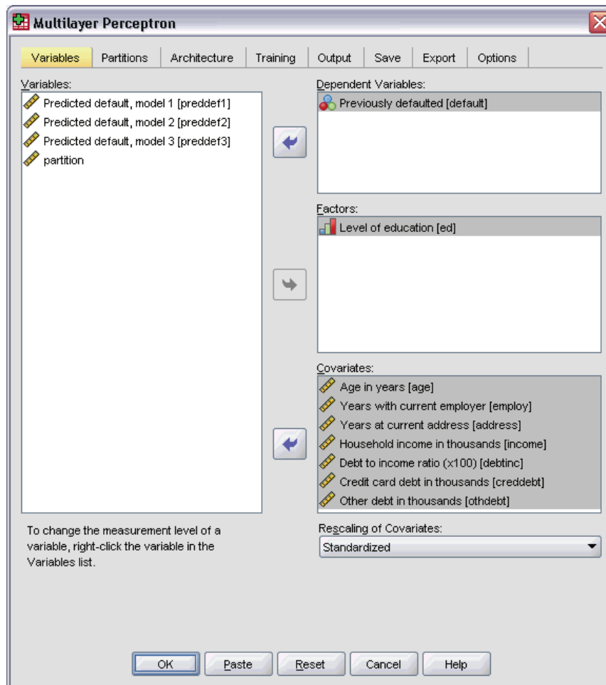
Figure 2-1 Multilayer Perceptron: Variables tab
