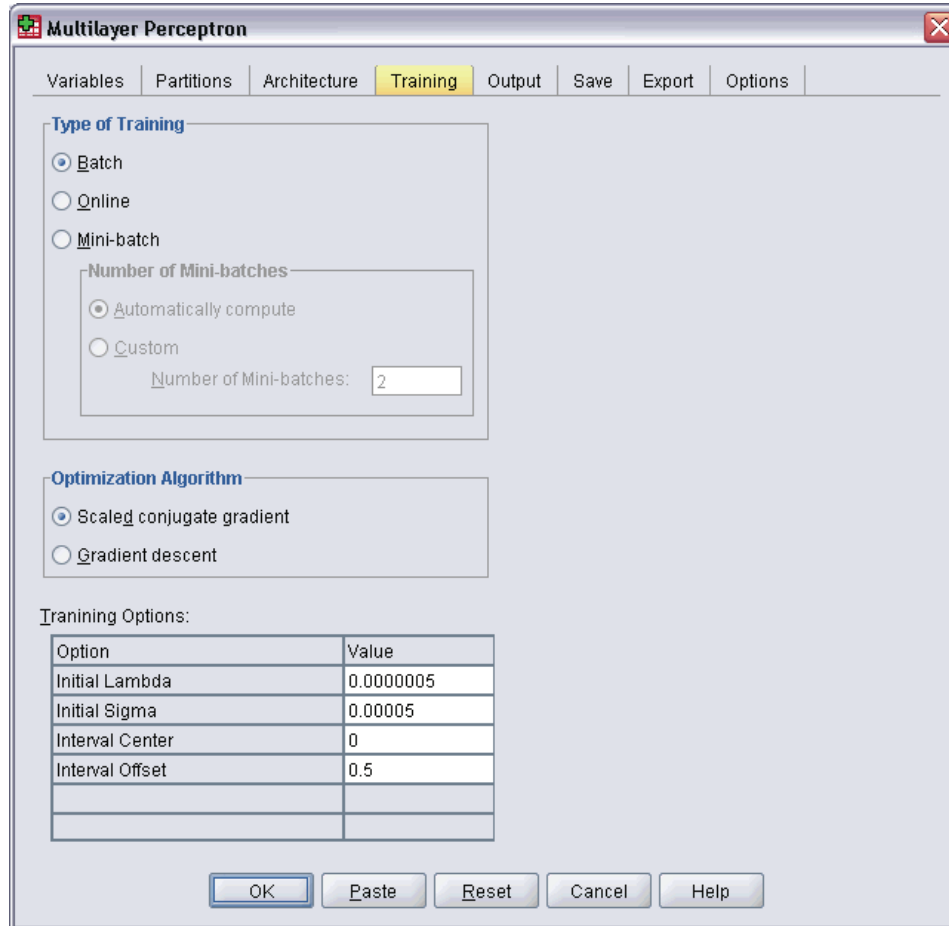
Figure 2-4 Multilayer Perceptron: Training tab
