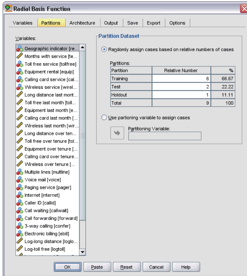
Figure 5-3 Radial Basis Function: Partitions tab
