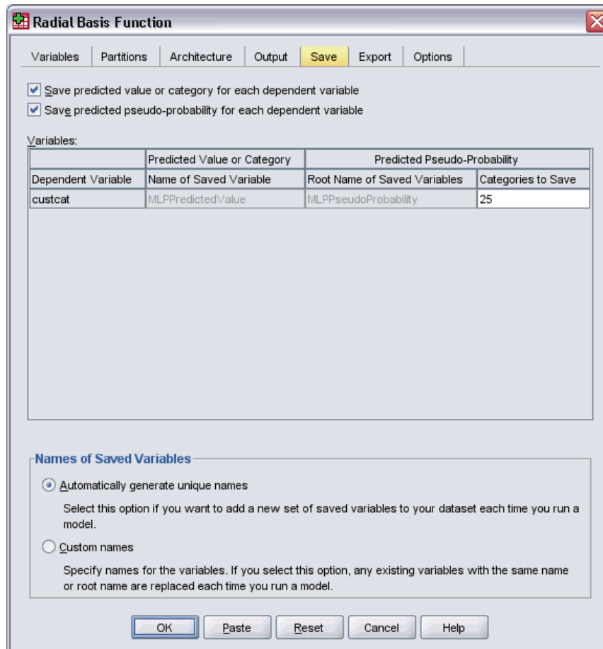
Figure 3-5 Radial Basis Function: Save tab
