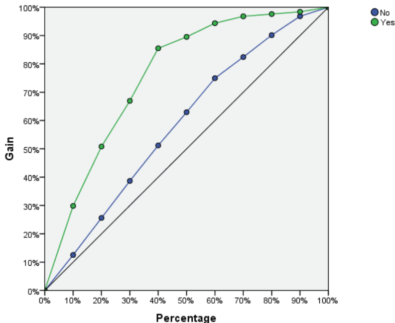
Figure 4-19 Cumulative gains chart
