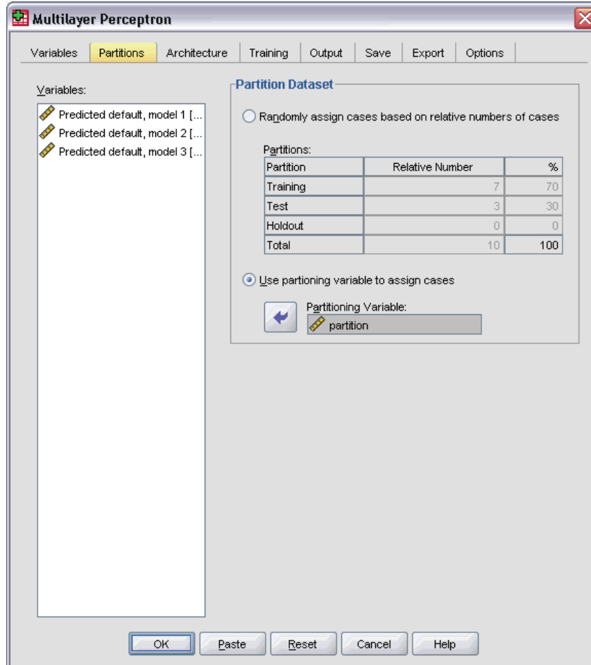
Figure 2-2 Multilayer Perceptron: Partitions tab
