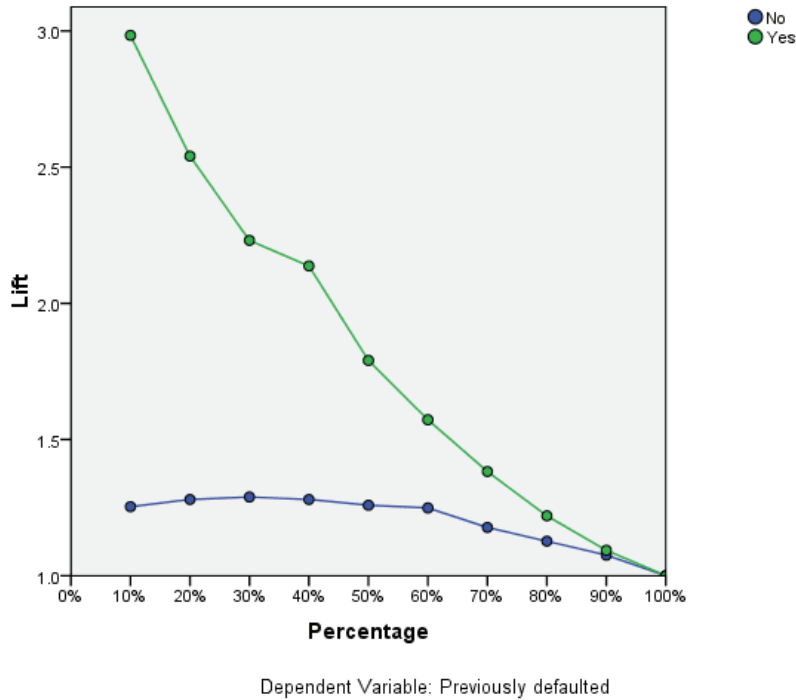
Figure 4-20 Lift chart
