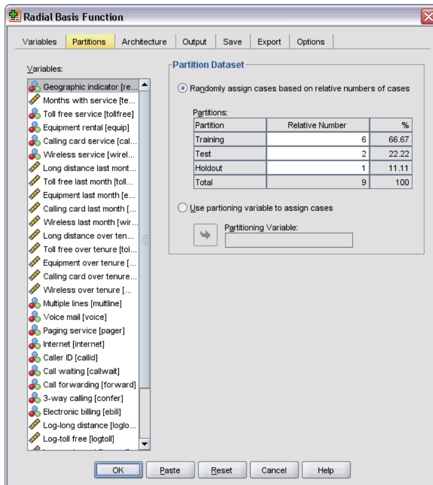
Figure 3-2 Radial Basis Function: Partitions tab
