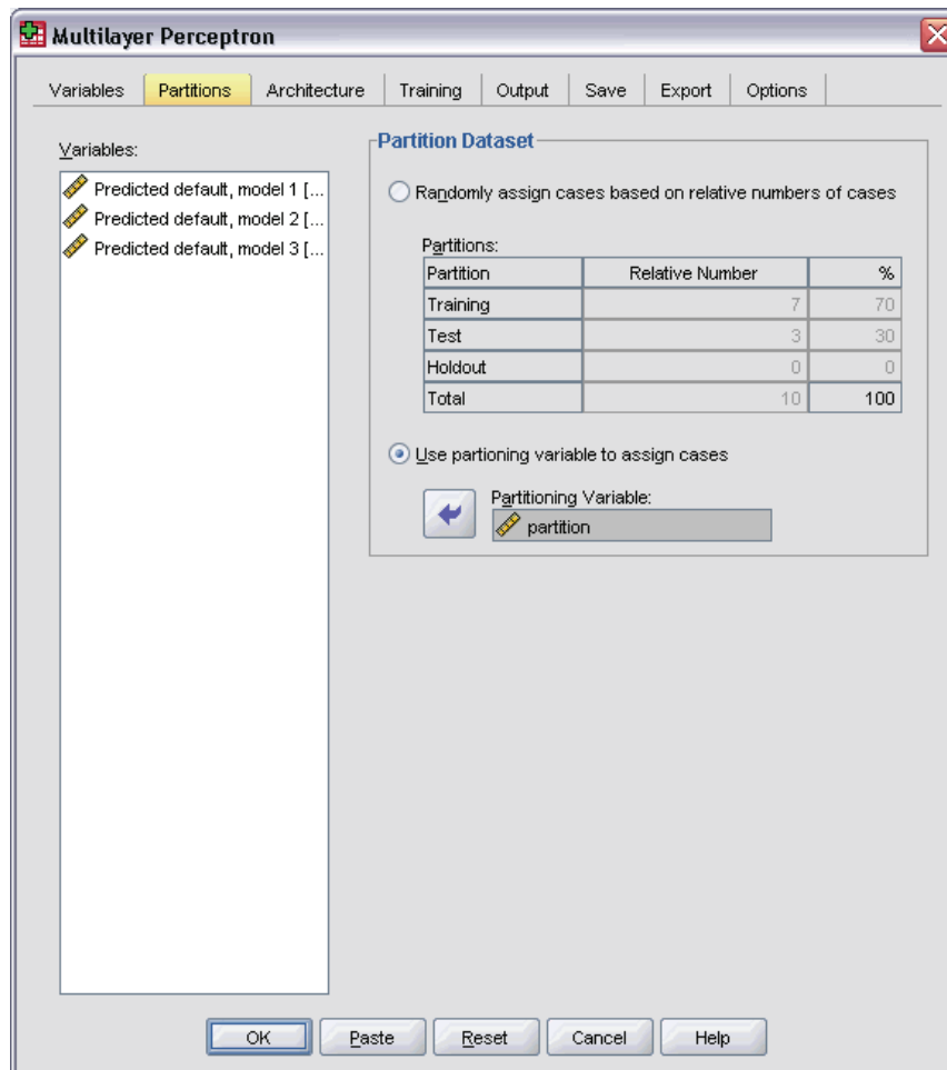
Figure 4-4 Multilayer Perceptron: Partitions tab
