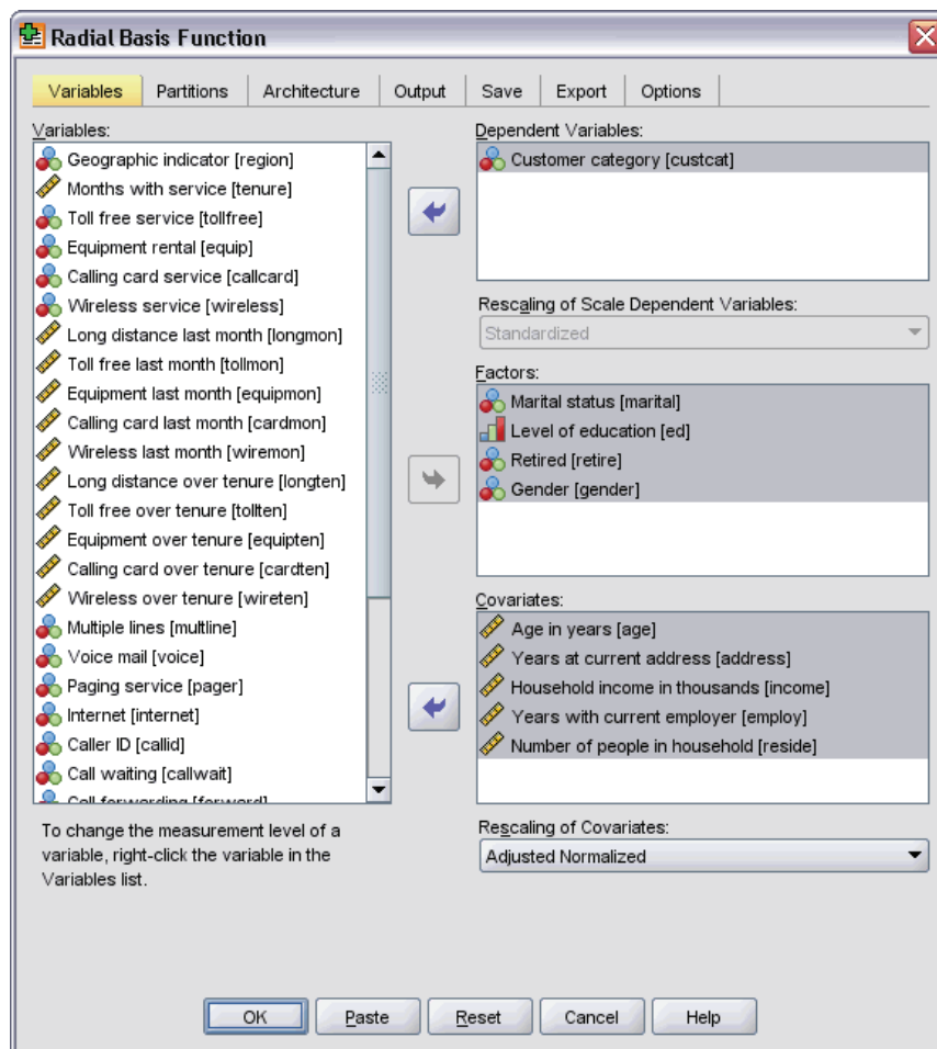
Figure 5-2 Radial Basis Function: Variables tab
