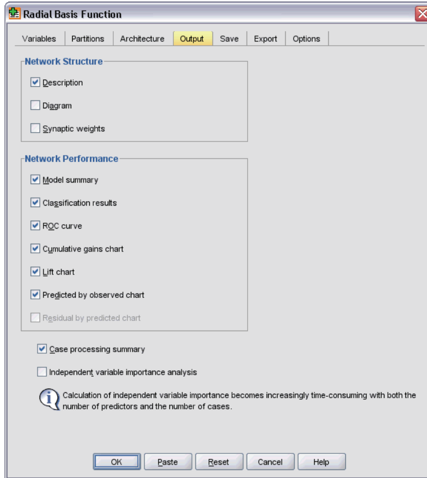
Figure 3-4 Radial Basis Function: Output tab
