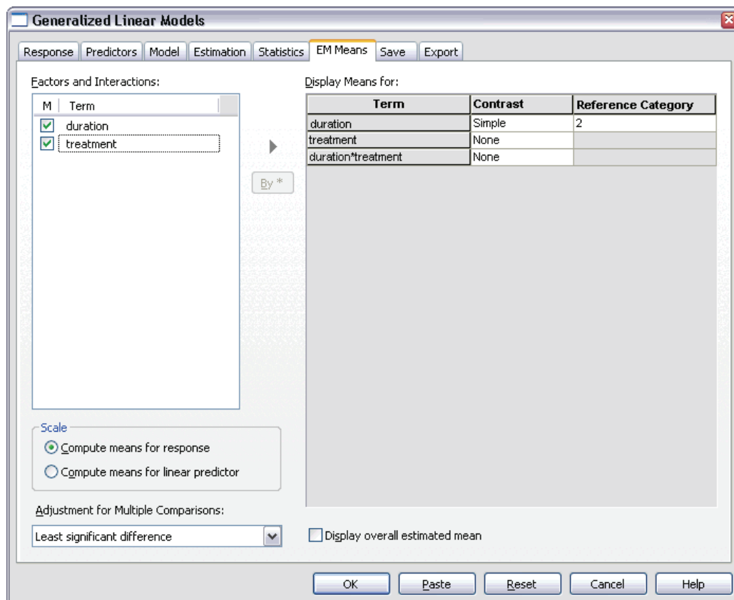
Figure 6-10 Generalized Linear Models: EM Means tab
