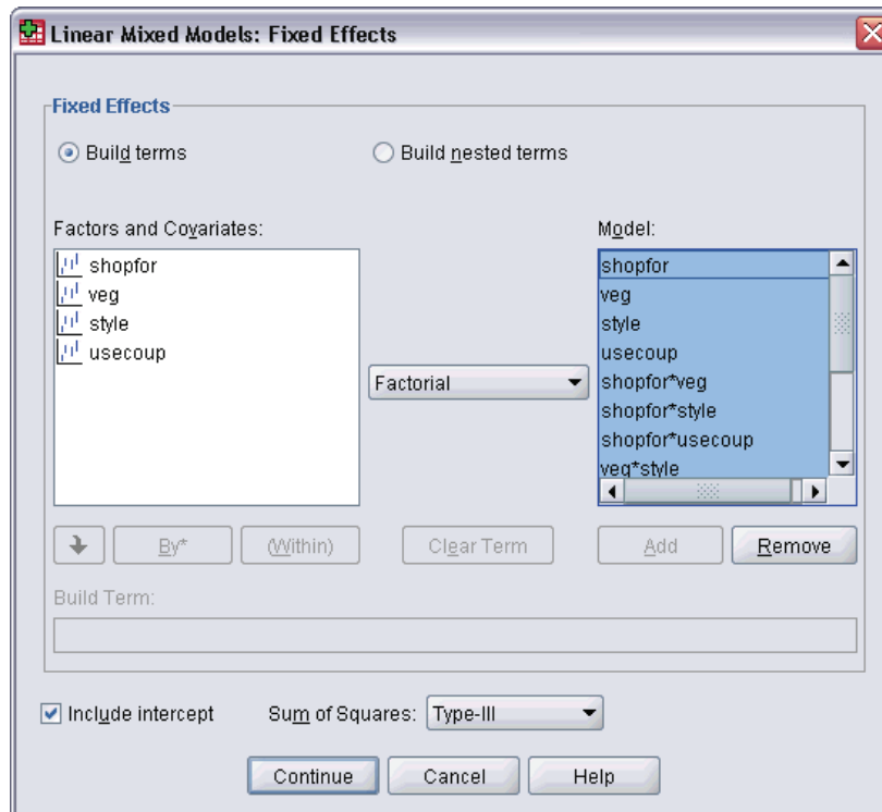
Figure 5-3 Linear Mixed Models Fixed Effects dialog box
