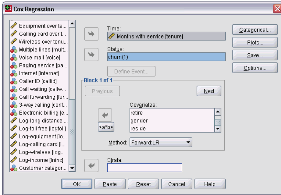
Figure 13-1 Cox Regression dialog box
