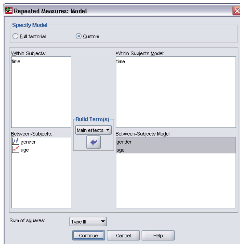
Figure 3-3 Repeated Measures Model dialog box
