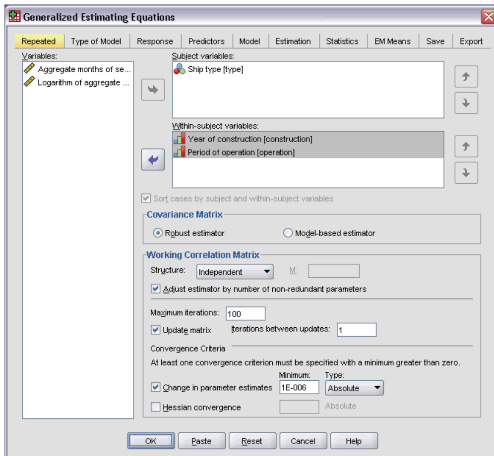
Figure 7-1 Generalized Estimating Equations: Repeated tab
