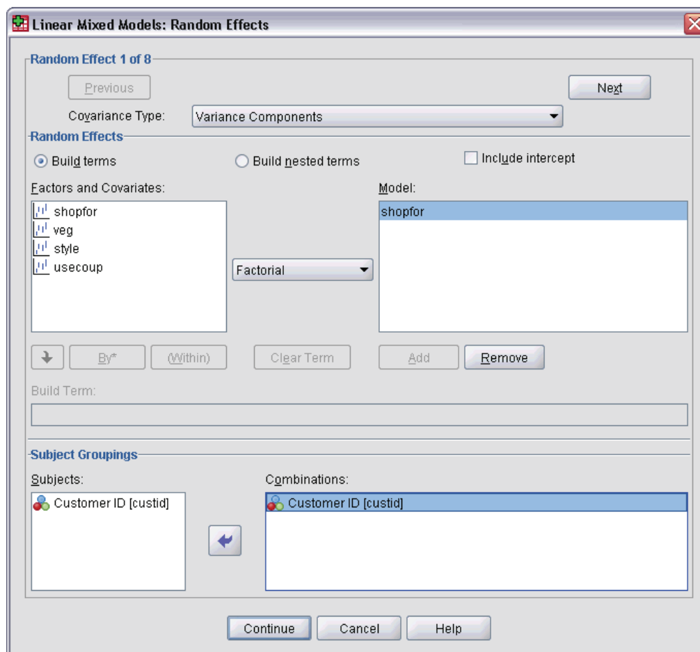
Figure 5-4 Linear Mixed Models Random Effects dialog box
