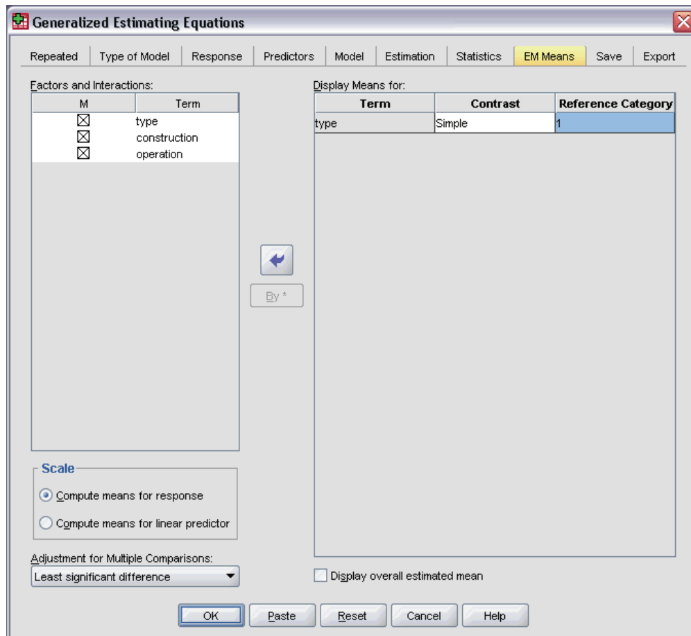
Figure 7-11 Generalized Estimating Equations: EM Means tab
