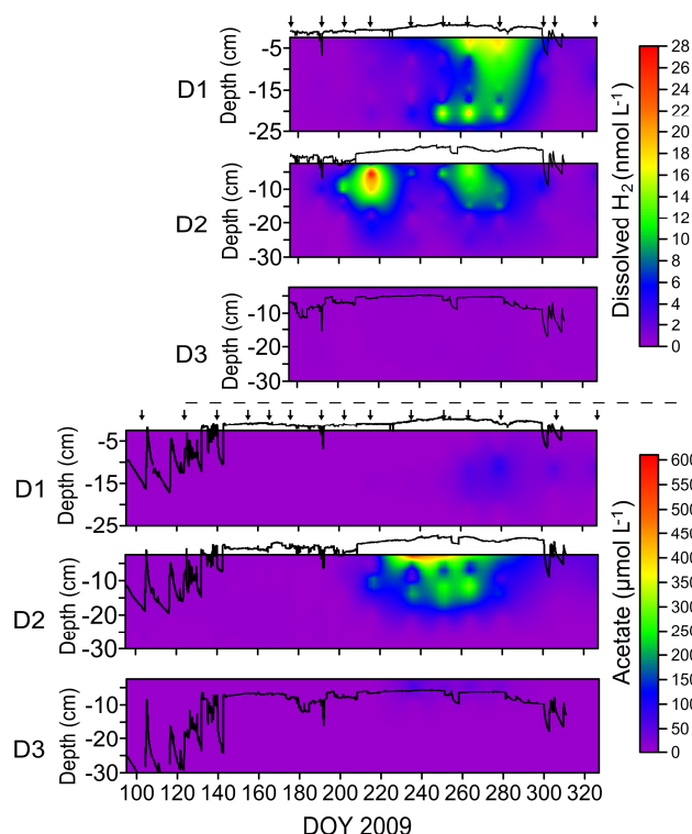
Fig. 9. Dissolved hydrogen and acetate concentrations during flooding (D plots). No or weak and sporadic accumulation occurred in C plots (see text).
