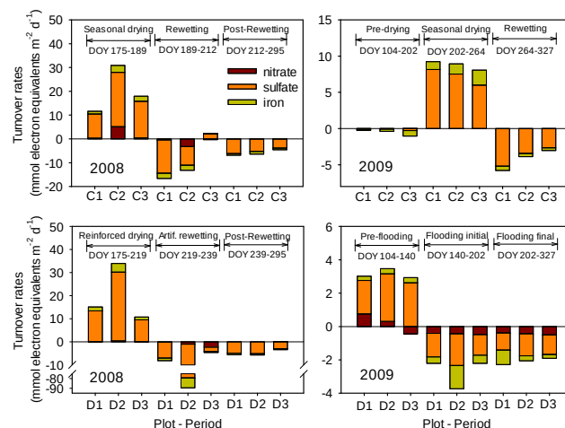
Fig. 10. Time-averaged net turnover rates of electron acceptors integrated for 30 cm profiles expressed in electron equivalents based on the dissolved concentrations measured (solutes) during different periods in all plots. Positive values refer to production (oxidation) and negative values to consumption (reduction).
